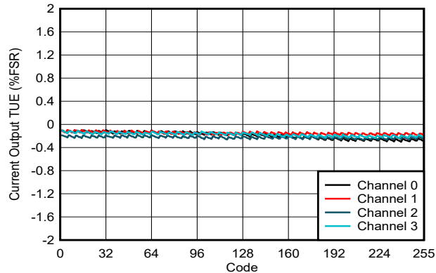
Figure 6-37. Current Output TUE vs Digital Input Code
