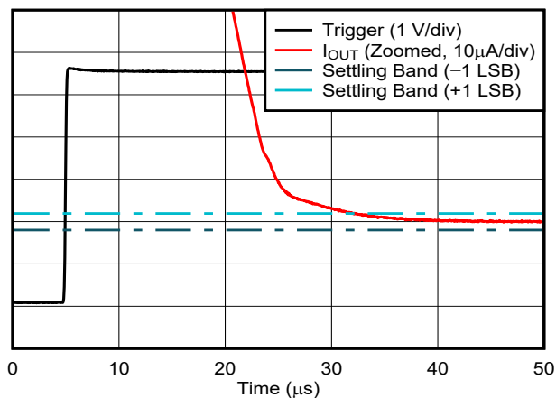
Figure 6-44. Current Output Setting Time, Falling Edge
