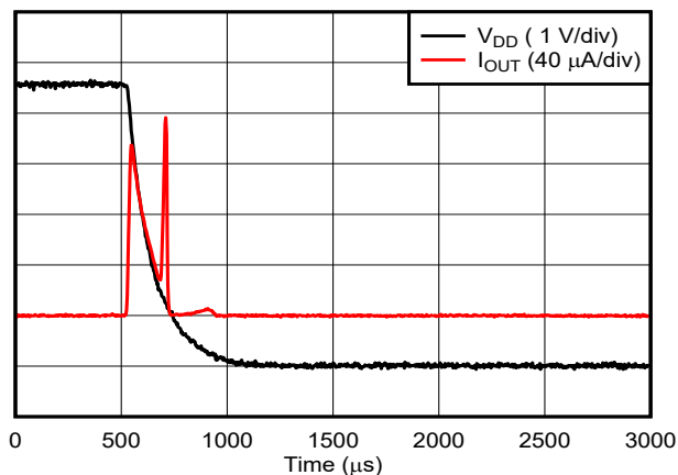
Figure 6-44. Current Output Setting Time, Falling Edge
