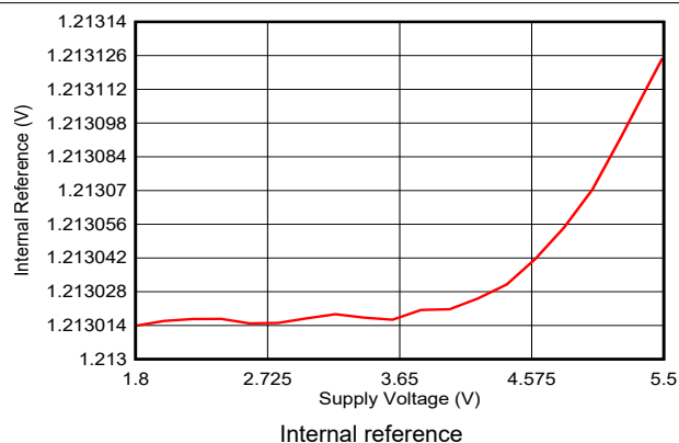
Figure 6-55. Internal Reference vs Supply Voltage
