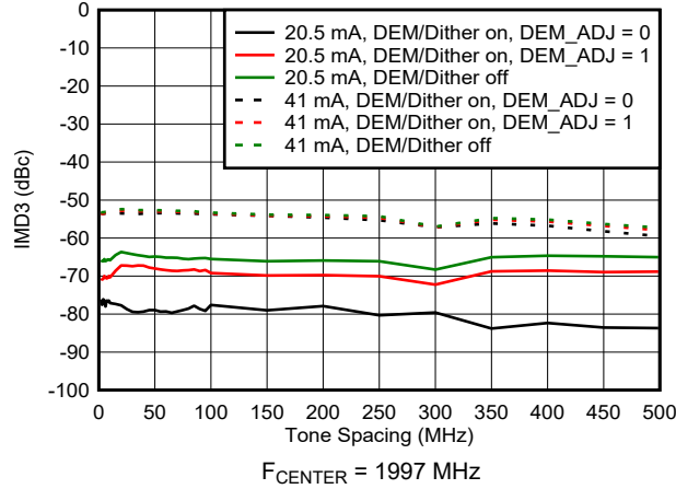
Figure 6-125. IMD3 vs Tone Spacing in NRZ Mode
