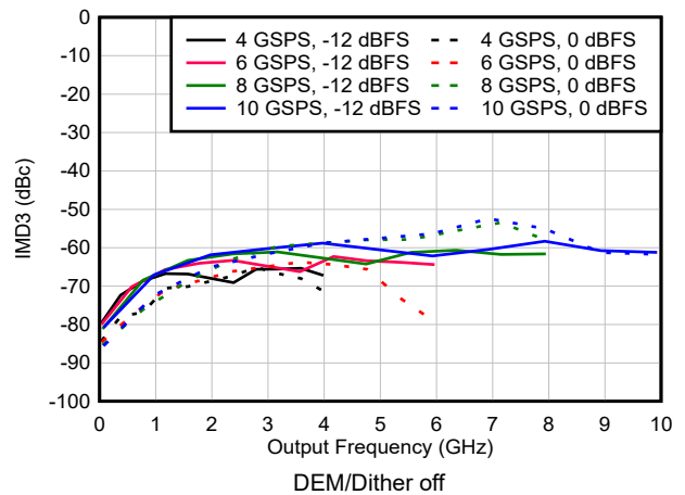
Figure 6-130. IMD3 vs Frequency and Sample Rate in NRZ/RF Modes
