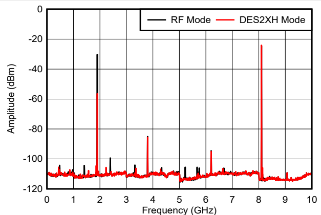
Figure 6-34. f_{\text{OUT}} = 8097\text{ MHz} , 0 dBFS
