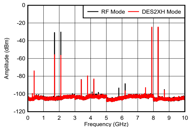
Figure 6-56. Dual Tone, f_{\text{OUT}} = 8097\text{ MHz} , -6 dBFS
