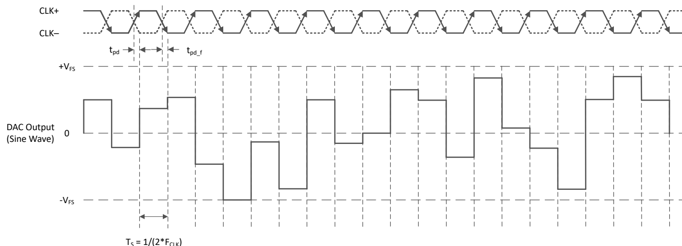
Figure 7-9. DES Mode Timing Diagram
