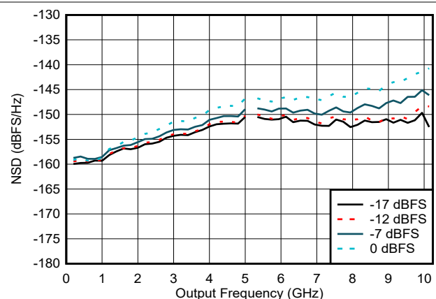
Figure 6-67. NSD vs Output Frequency and Digital Amplitude
