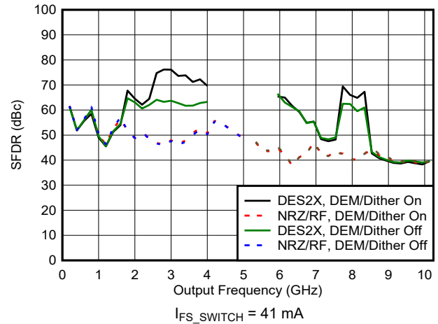
Figure 6-90. SFDR vs Frequency and Mode
