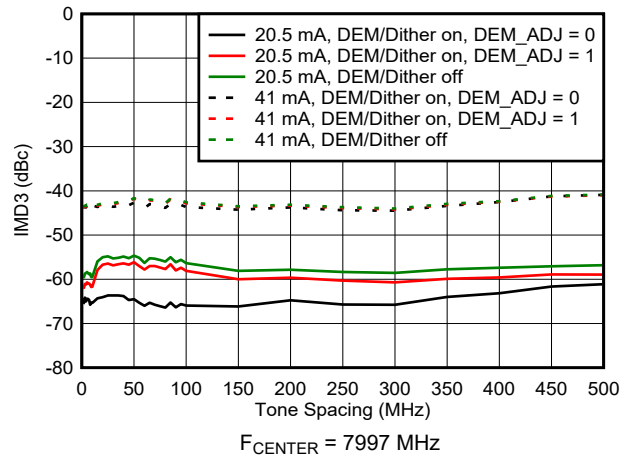
Figure 6-128. IMD3 vs Tone Spacing in DES2XH Mode
