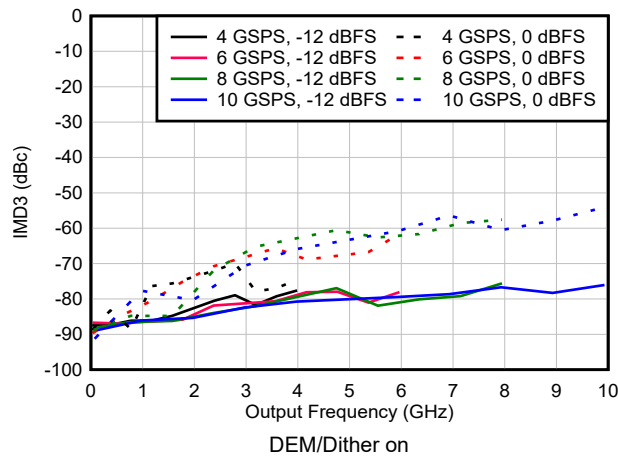
Figure 6-129. IMD3 vs Frequency and Sample Rate in NRZ/RF Modes
