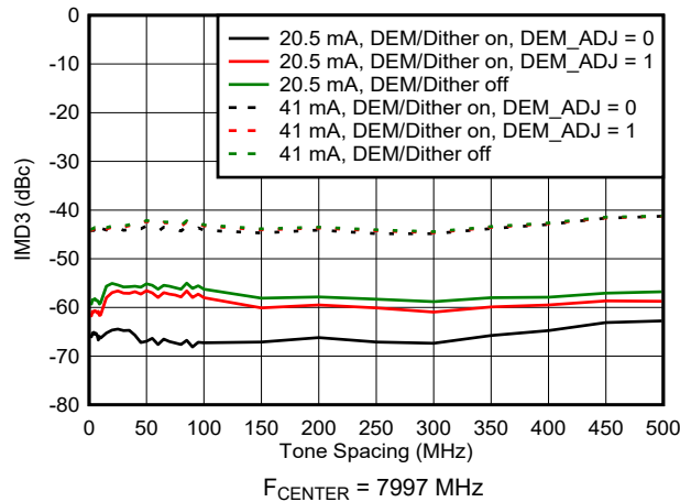
Figure 6-127. IMD3 vs Tone Spacing in RF Mode
