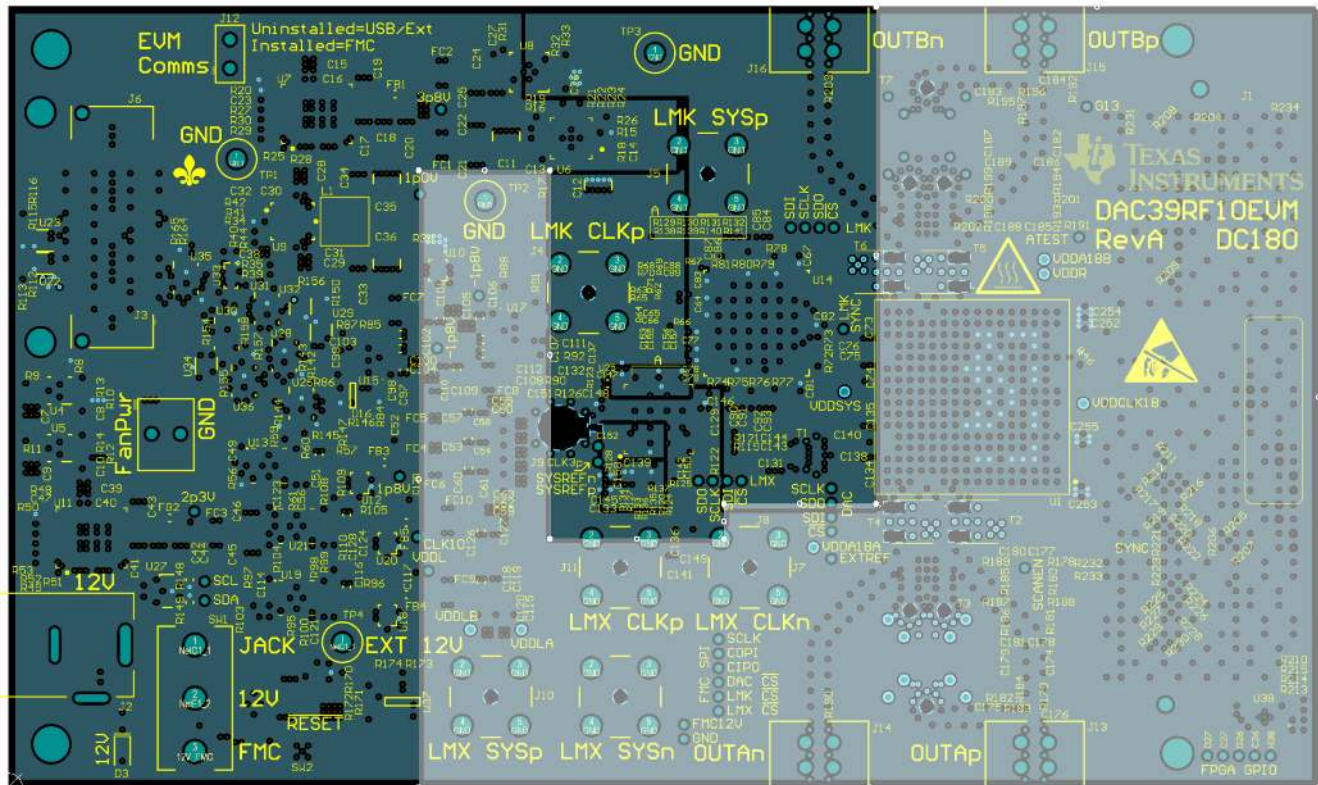
Layer3 / PWR1 DAC DVDD = WHITE Other PWR Planes = AUX Supplies Figure 8-31. Power Plane Layout for Layer 3
