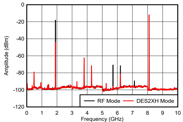
Figure 6-32. f_{\text{OUT}} = 6097\text{ MHz} , -6 dBFS
