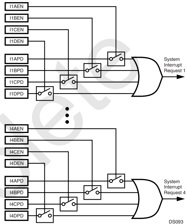
Figure 71. VTU Interrupt Request Structure
