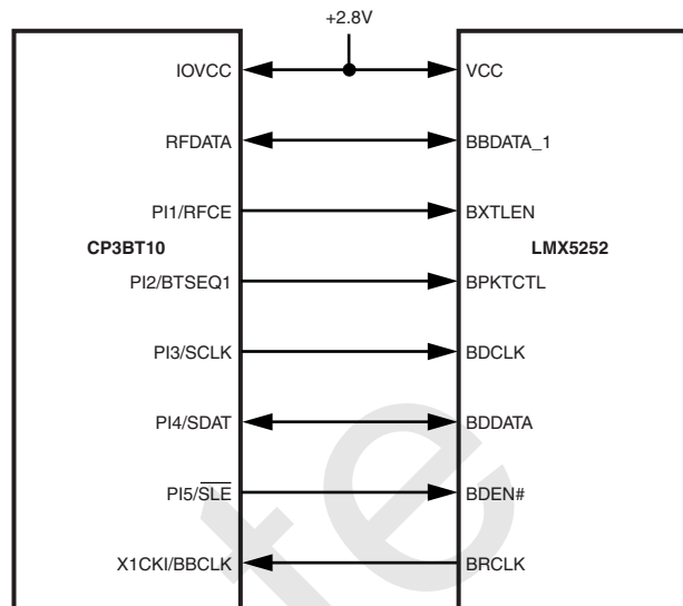
Figure 13. LMX5252 Interface
