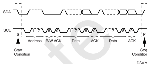
Figure 59. A Complete ACCESS.bus Data Transaction
