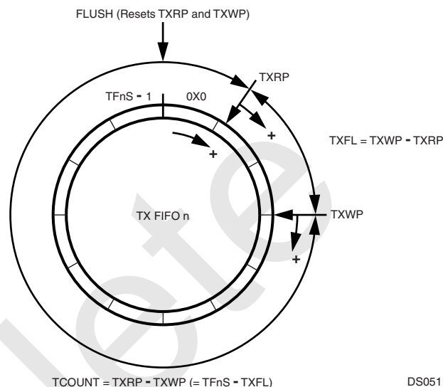
Figure 27. Transmit FIFO Operation
