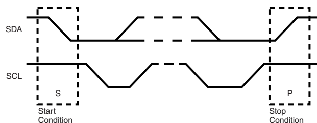
Figure 56. Start and Stop Conditions
