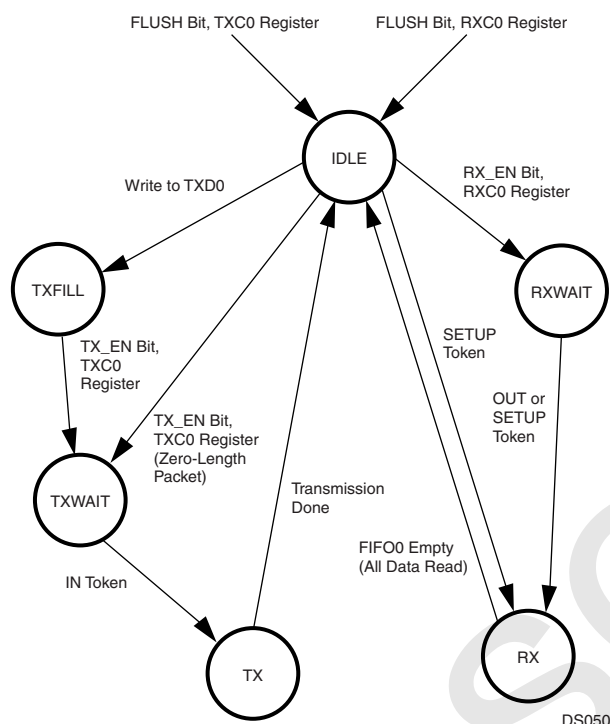
Figure 26. Endpoint 0 Operation
