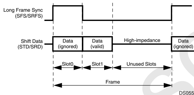
Figure 32. Network Mode Frame
