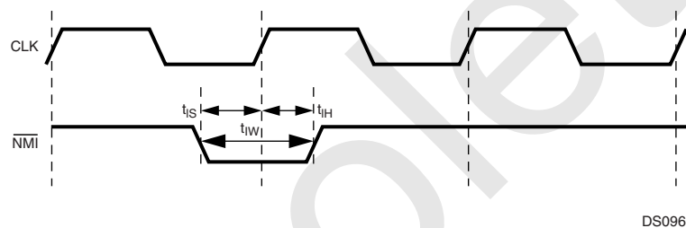
Figure 73. \overline{\text{NMI}} Signal Timing
