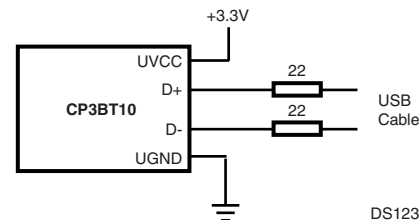
Figure 29. USB Transceiver Interface
