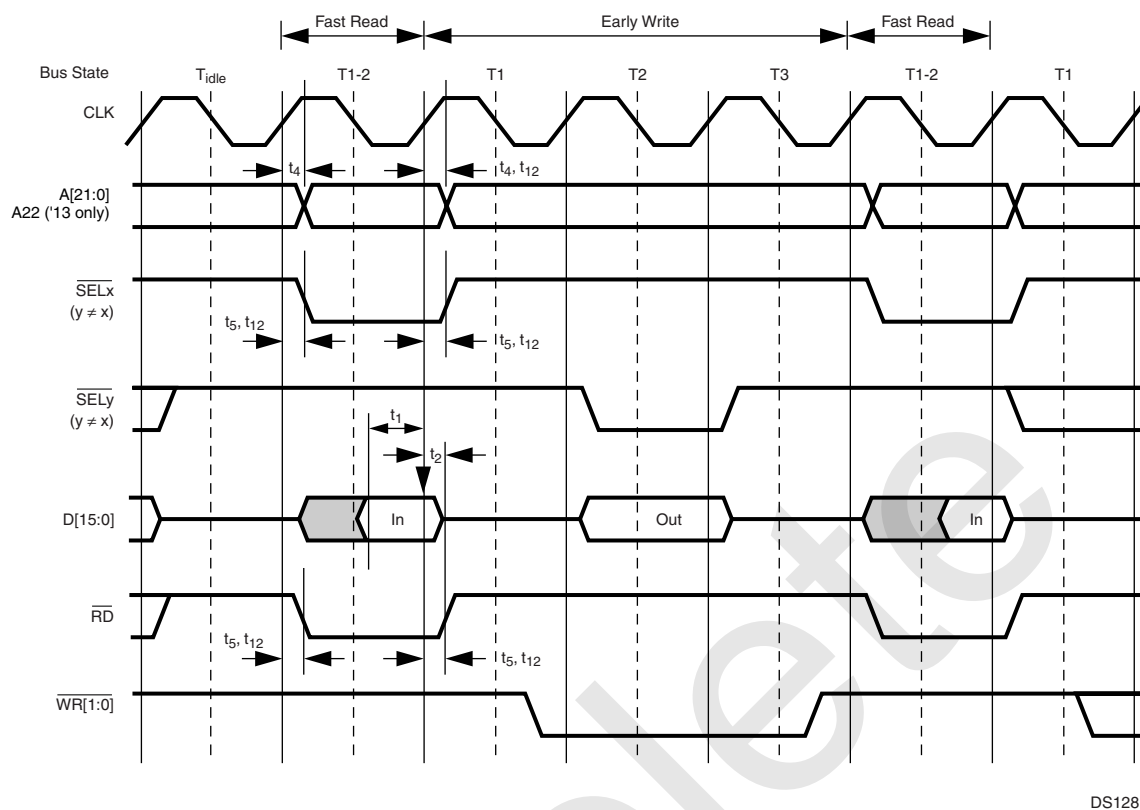
Figure 96. Early Write Between Fast Read Cycles
