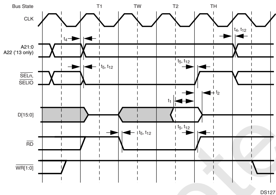
Figure 95. Normal Read Cycle (Wait Cycle Followed by Hold Cycle)
