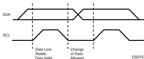
Figure 55. Bit Transfer
