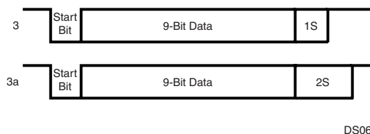
Figure 45. 9-bit Data Frame Options
