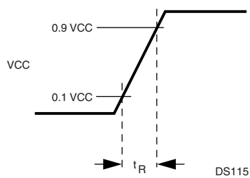
Figure 75. Power-On Reset
