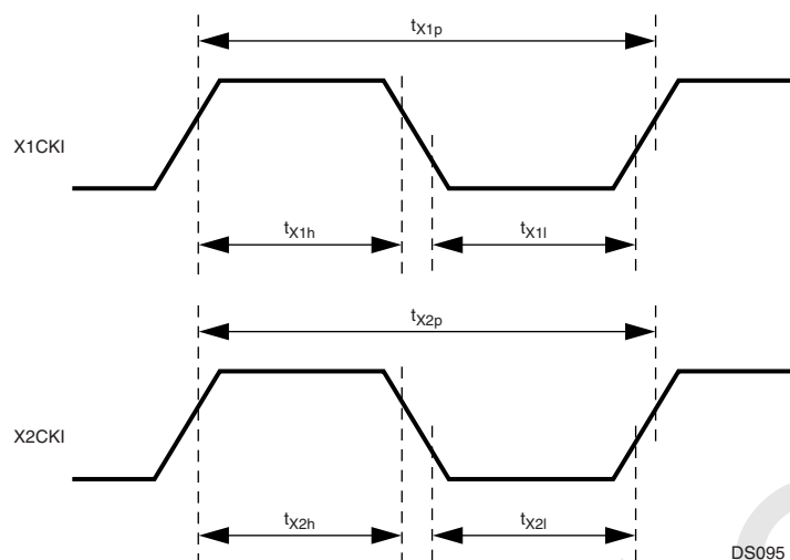
Figure 72. Clock Timing
