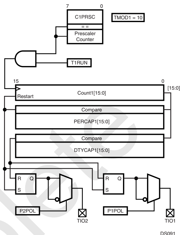
Figure 69. VTU 16-bit PWM Mode
