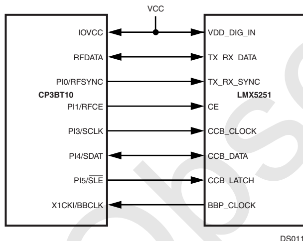
Figure 12. LMX5251 Interface
