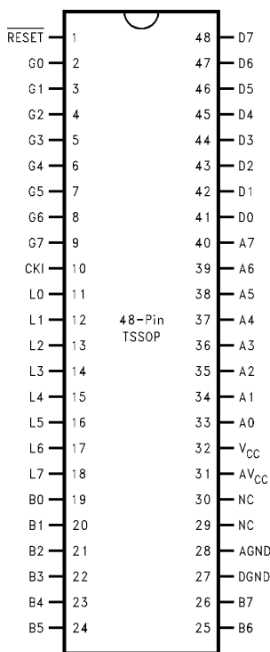
Figure 2-5. TSSOP Package (Top View) See Package Number DGG0056A
