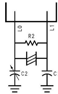
Low Speed Oscillator
