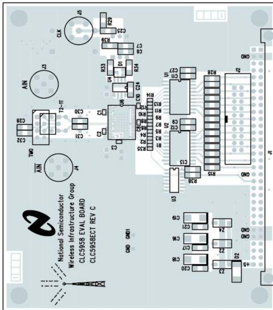
Figure 29. CLC5958PCASM Layer 1
