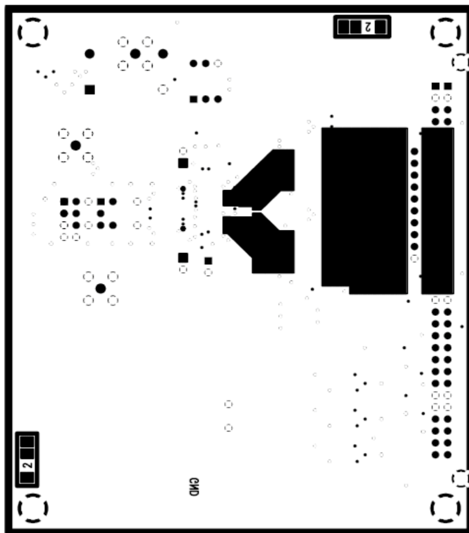
Figure 30. CLC5958PCASM Layer 2
