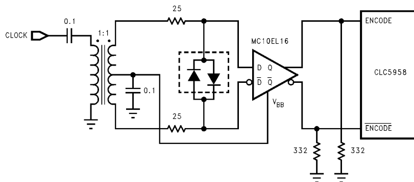
Figure 25. Encode Inputs
