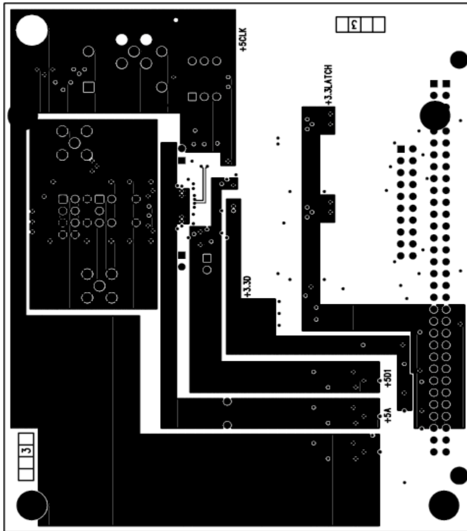
Figure 31. CLC5958PCASM Layer 3
