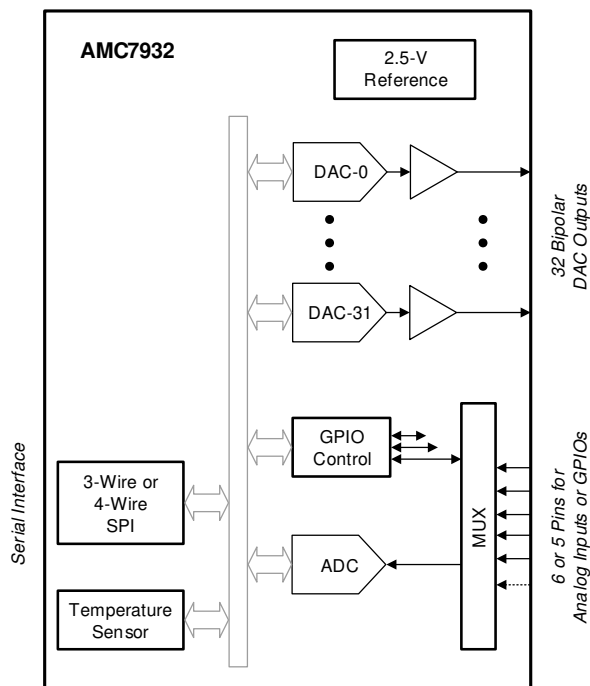
Simplified Schematic
