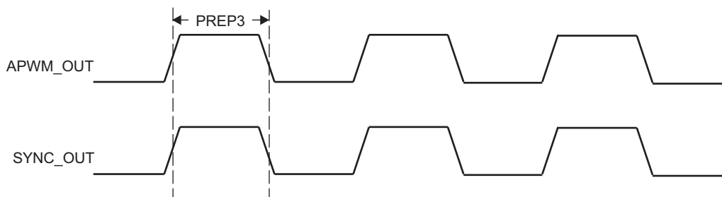
Figure 6-65. PRU-ICSS ECAP Switching Characteristics
