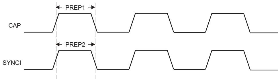
Figure 6-64. PRU-ICSS ECAP Timing
