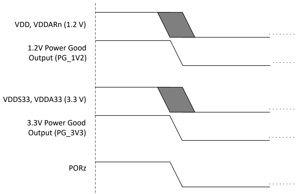
Figure 6-2. Power-Down Sequencing
