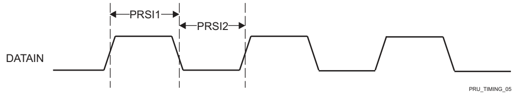
Figure 6-53. PRU-ICSS PRU Shift In Timing
