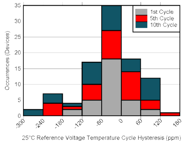
Figure 5-37. Multiple Temperature Cycle Hysteresis
