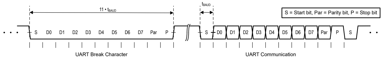
Figure 5-2. UBM Timing
