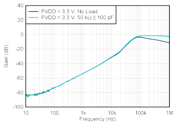
Figure 5-27. DAC AC PSRR vs Frequency
