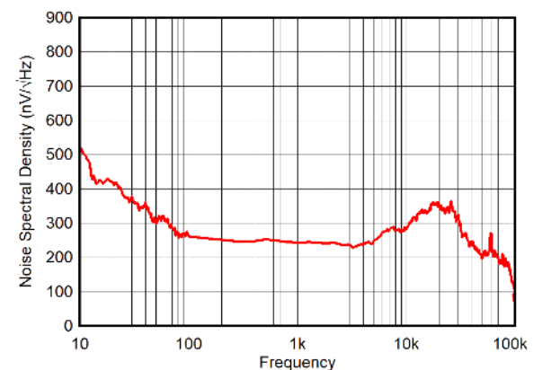
Figure 5-20. DAC Output Noise Density vs Frequency
