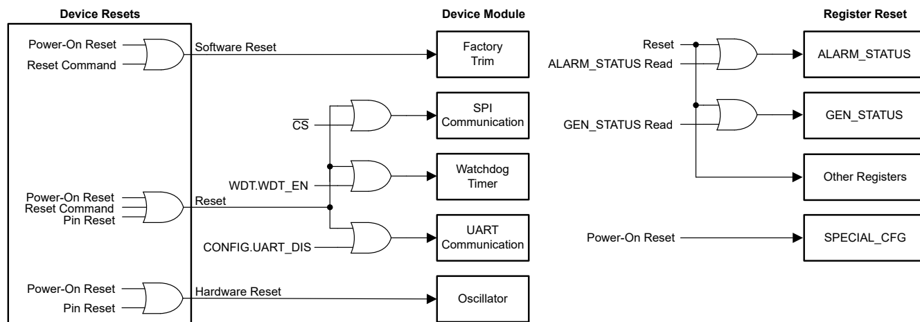
Figure 6-16. Reset Conditions
