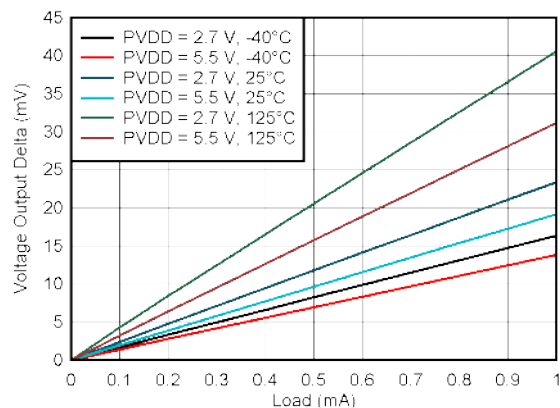
Figure 5-9. Zero-code Impedance
