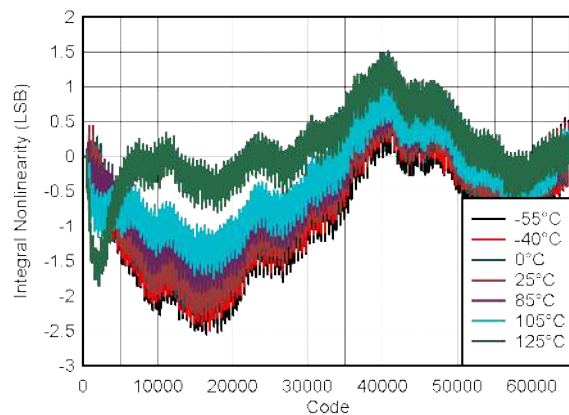
Figure 5-5. DAC INL vs Digital Input Code
