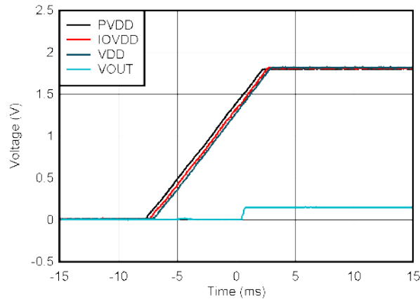
Figure 6-27. DAC Supply Power On, PVDD = 1.8 V
