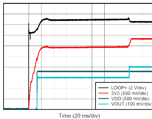
Figure 8-7. Circuit Start-Up
