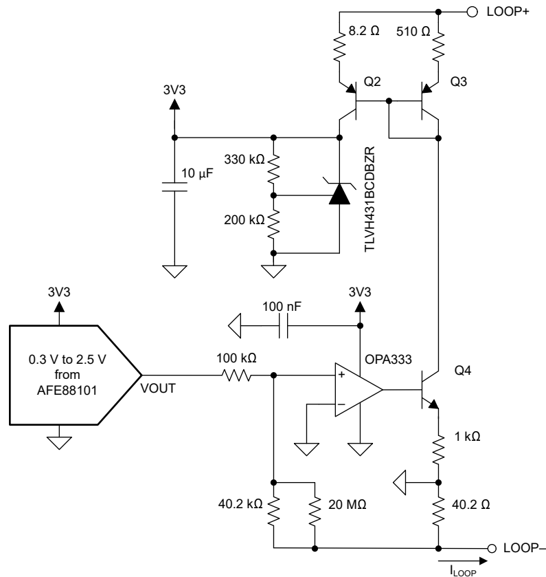
In this circuit, the VOUT voltage is set across the 100-k \Omega resistor by the AFE88101. The opposite end of the 100-k \Omega resistor is set to ground by the feedback of the OPA333. The current across the 100-k \Omega resistor is VOUT divided by 100 k \Omega . This current continues through the 40.2-k \Omega resistor so that the voltage at LOOP– is less than ground. Equation 11 calculates the voltage at LOOP–.
