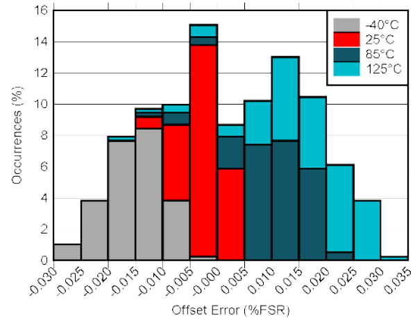
Figure 6-16. DAC Offset Error vs Temperature
