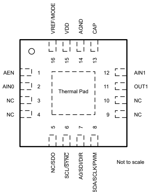
Figure 5-3. AFE439A2: RTE Package, 16-pin WQFN (Top View)
