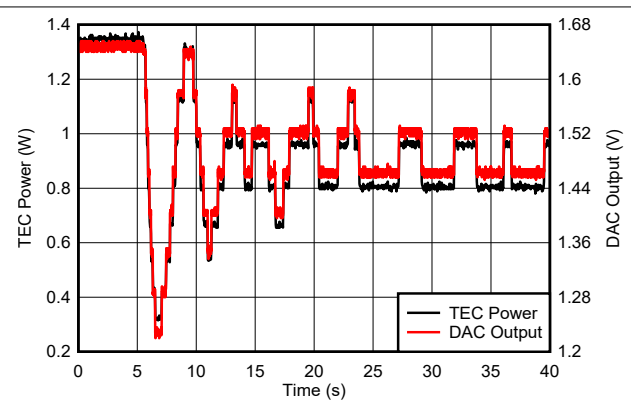
Figure 8-3. TEC Power and DAC Output vs Time
