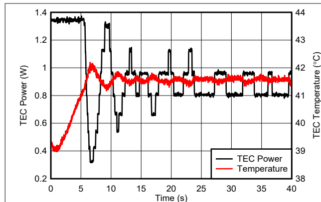
Figure 8-2. TEC Power and TEC Temperature vs Time
