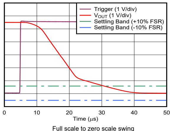
Figure 6-22. Voltage Output Setting Time - Falling Edge
