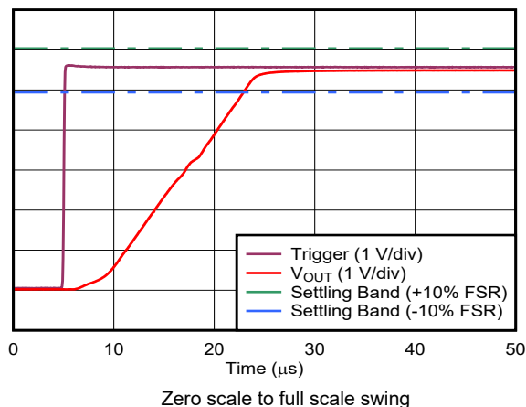
Figure 6-21. Voltage Output Settling Time - Rising Edge
