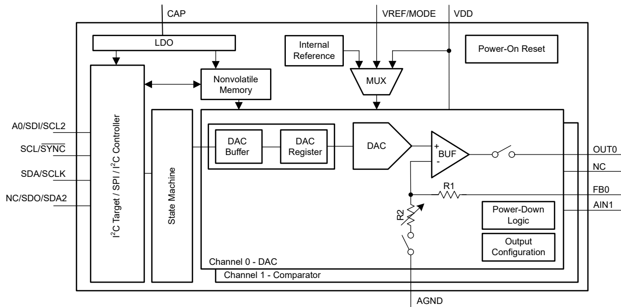
Figure 7-3. Functional Block Diagram: AFE639D2
