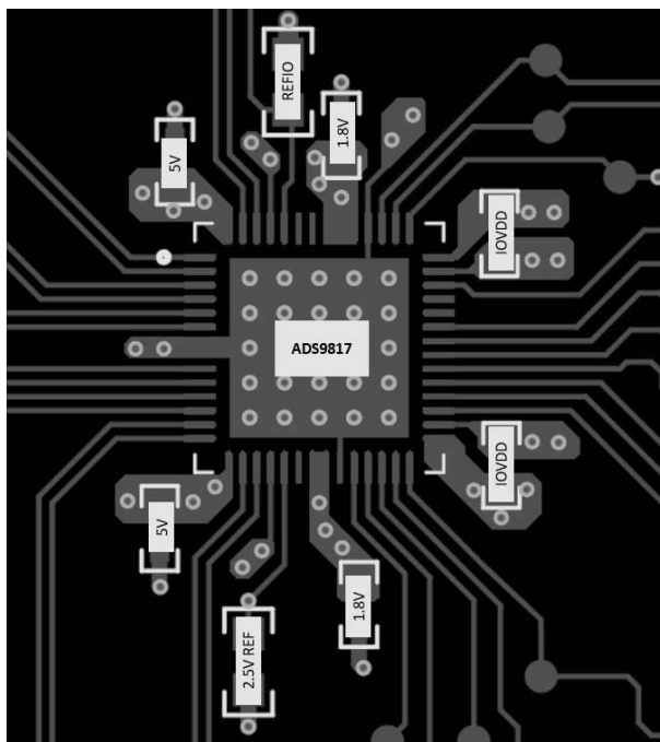
Figure 8-5. Example Layout
