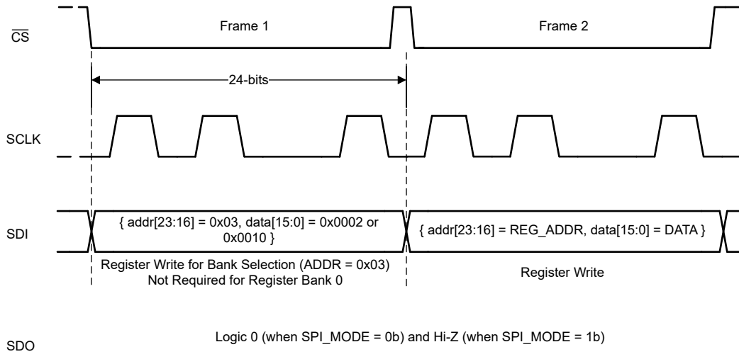
Figure 6-10. Register Write
