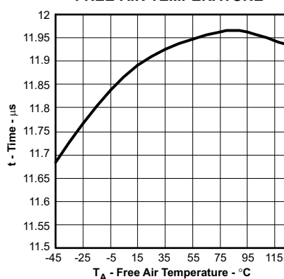
Figure 29. INL
