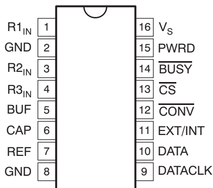
DW PACKAGE SO-16 (TOP VIEW)
