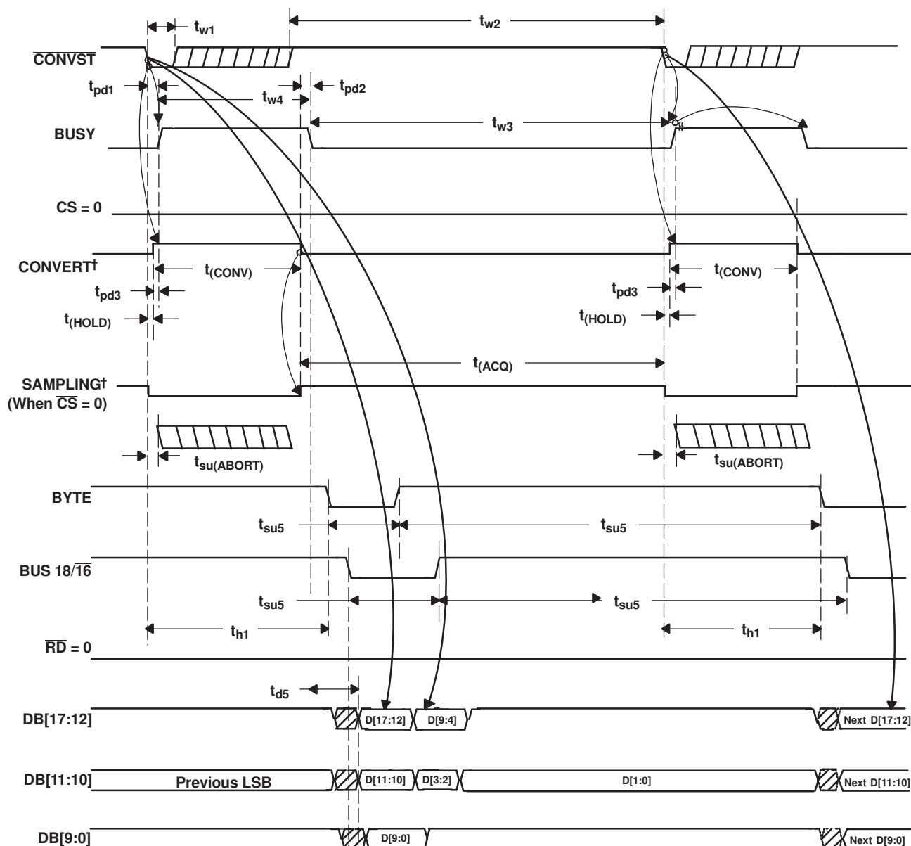
Figure 34. Timing for Conversion and Acquisition Cycles With \overline{\text{CS}} and \overline{\text{RD}} Tied to BDGND - Auto Read
