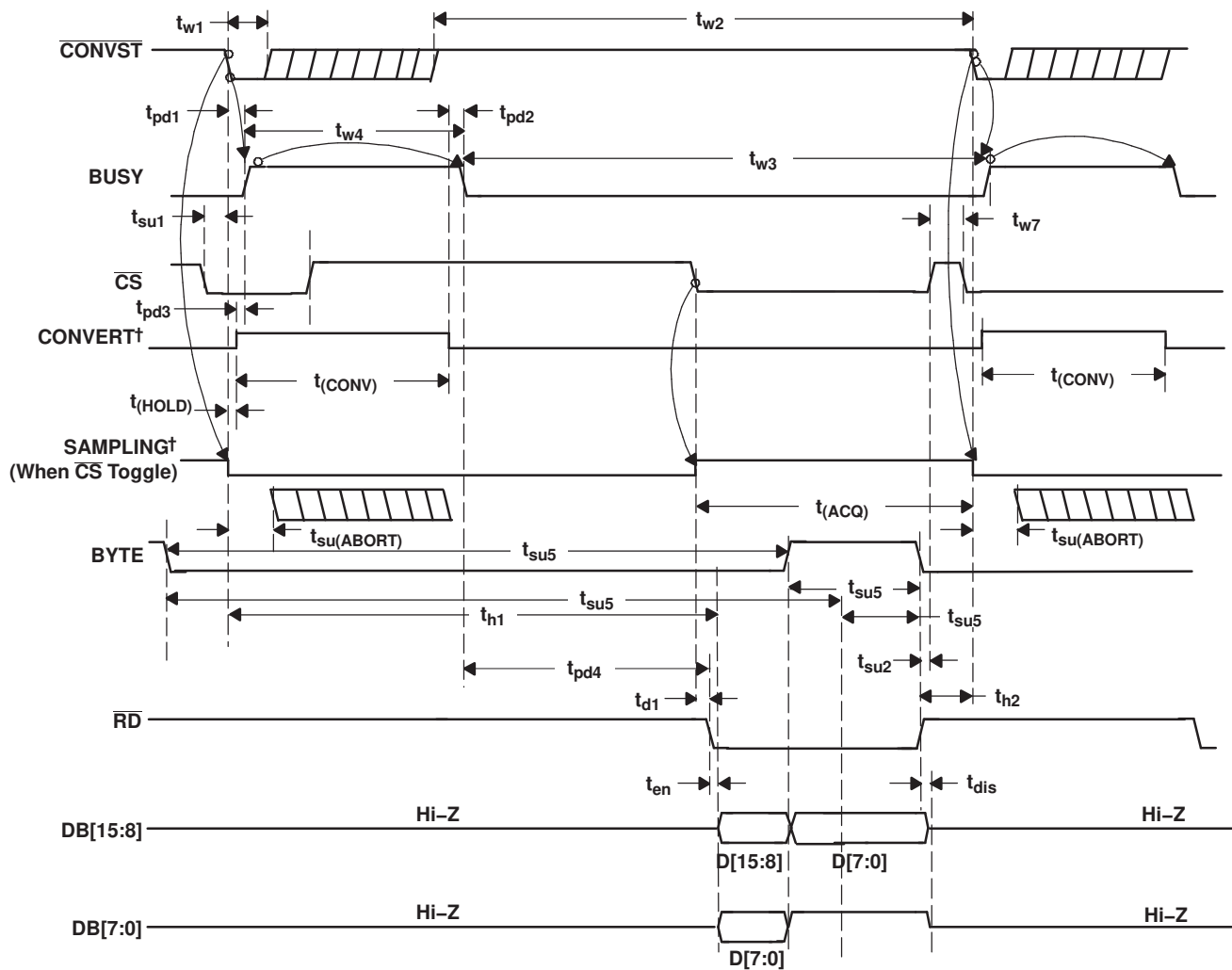
Figure 32. Timing for Conversion and Acquisition Cycles With \overline{\text{CS}} and \overline{\text{RD}} Toggling
