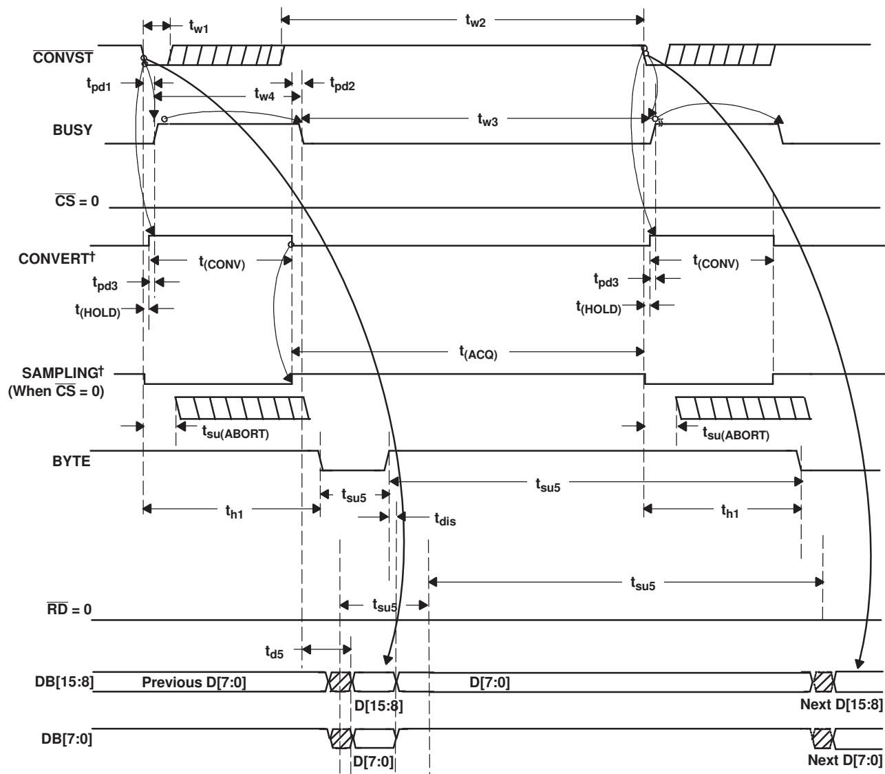
Figure 35. Timing for Conversion and Acquisition Cycles With \overline{\text{CS}} and \overline{\text{RD}} Tied to BDGND - Auto Read
