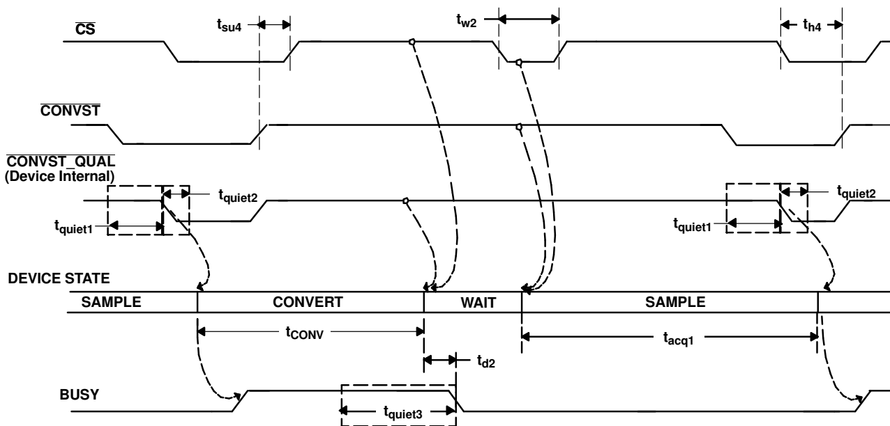
Figure 44. Convert and Sample with Wait
