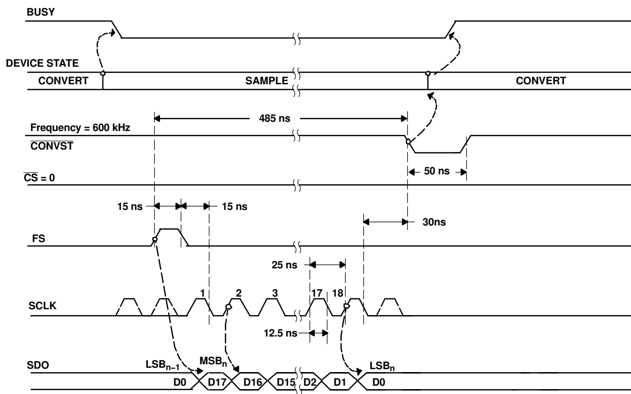
Figure 59. Example Stimulus in Serial Interface With FS Active, Back-To-Back Conversion that Achieves 600 KSPS
