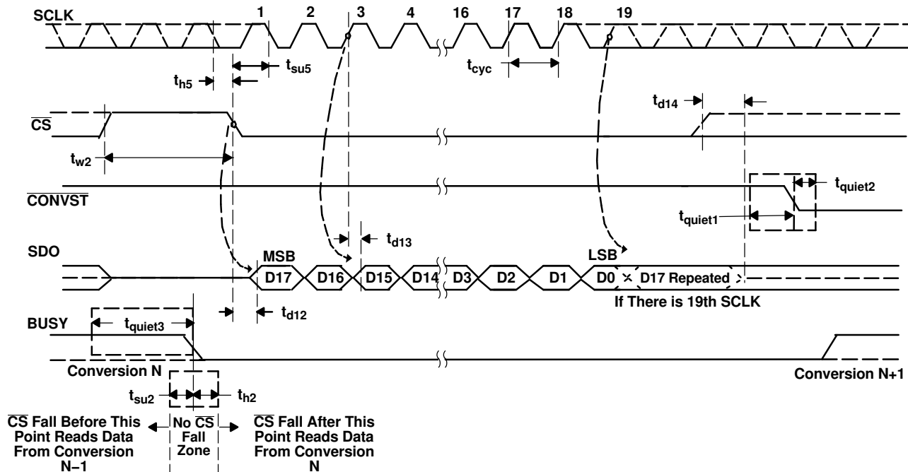
Figure 47. Read Frame Controlled via \overline{\text{CS}} (FS = 1)
