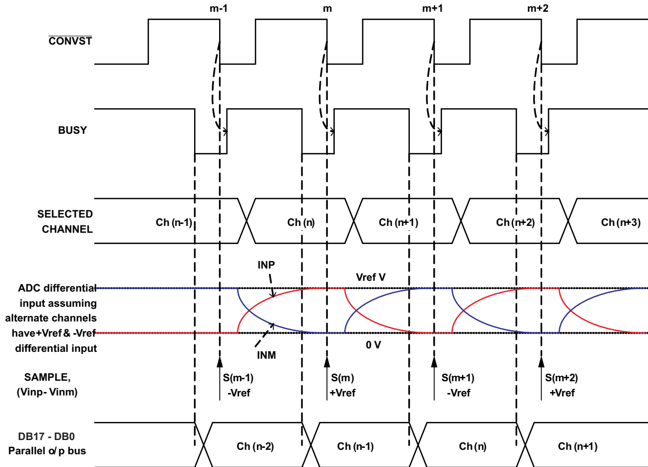
Figure 1. Device Operation
