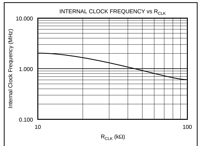
FIGURE 15. Internal Clock Frequency vs R_{\text{CLK}} Resistor Value.
