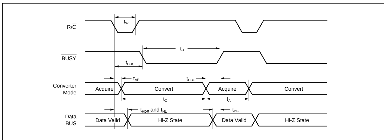
FIGURE 6. Convert Mode: \overline{\text{R}/\text{C}} Pulse LOW — Outputs Enabled After Conversion.
