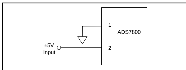
FIGURE 5. \pm 5\text{V} Range Without Trims.
