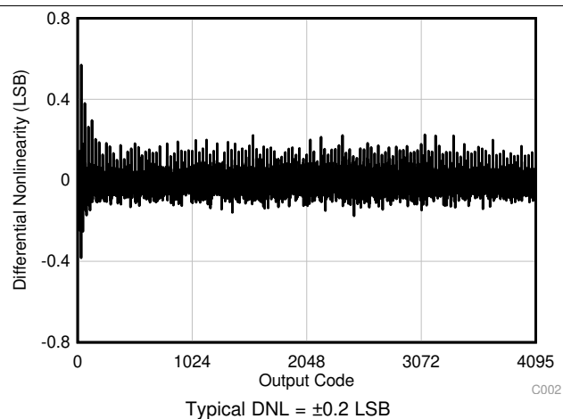
Figure 3. Typical DNL
