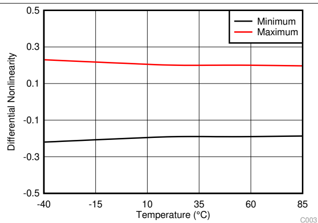
Figure 3. Typical DNL
