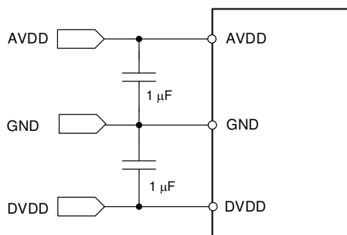
Figure 8-3. Power-Supply Decoupling
