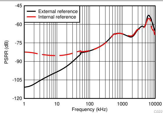
Figure 6-22. PSRR vs Frequency
