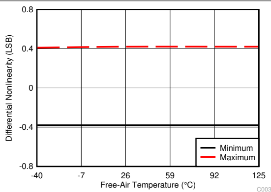
Figure 6-3. Typical DNL
