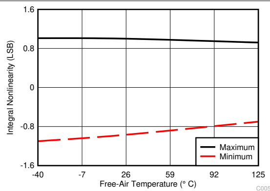
Figure 6-4. Typical INL
