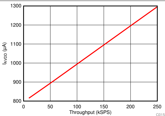
Figure 6-21. Analog Supply Current vs Throughput
