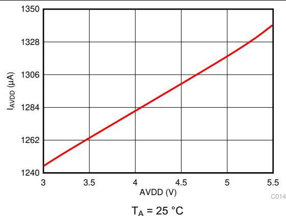
Figure 6-20. Analog Supply Current vs AVDD
