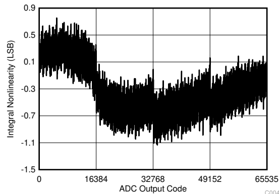
Figure 6-4. Typical INL
