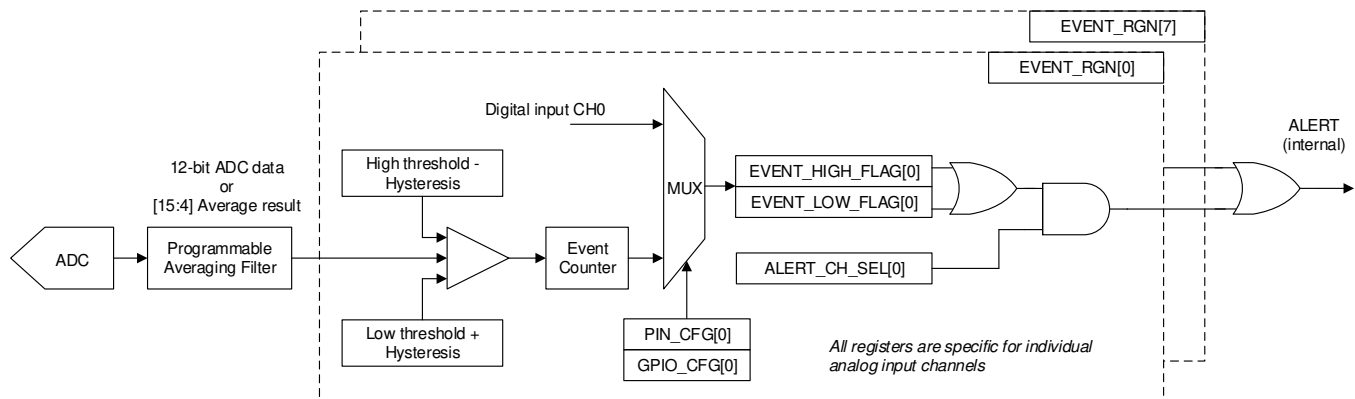
Figure 27. Digital Window Comparator Block Diagram
