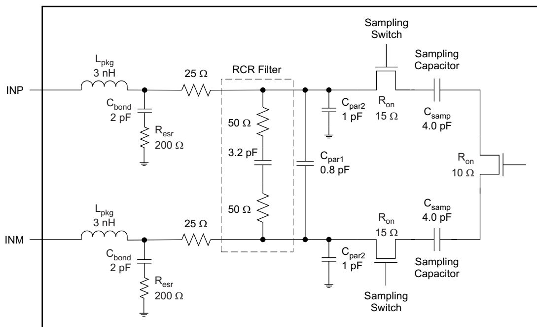
Figure 82. Input Sampling Circuit
