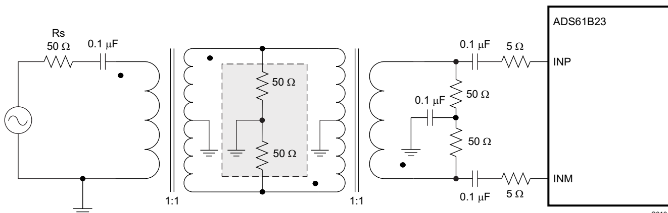
Figure 35. Two Transformer Drive Circuit
