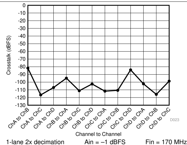
Figure 28. Crosstalk by Channel
