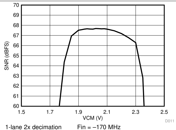
Figure 15. SNR vs. VCM
