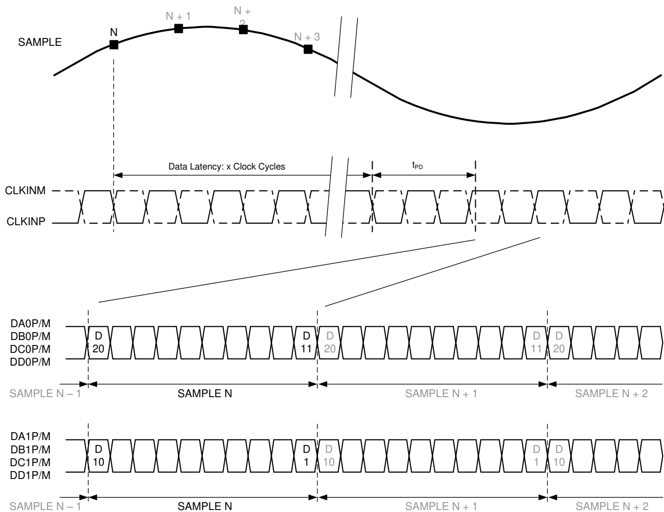
Figure 3. Timing Diagram: 500 MSPS Output Data Rate
