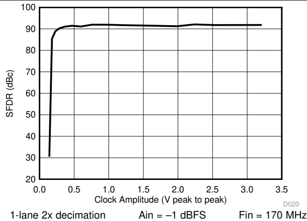
Figure 24. SFDR vs. Clock Amplitude
