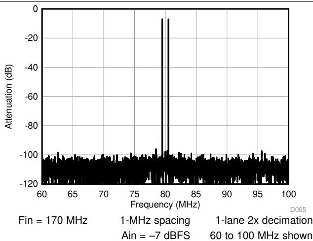
Figure 26. 2-Tone FFT
