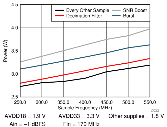
Figure 27. Power vs. Sample Frequency
