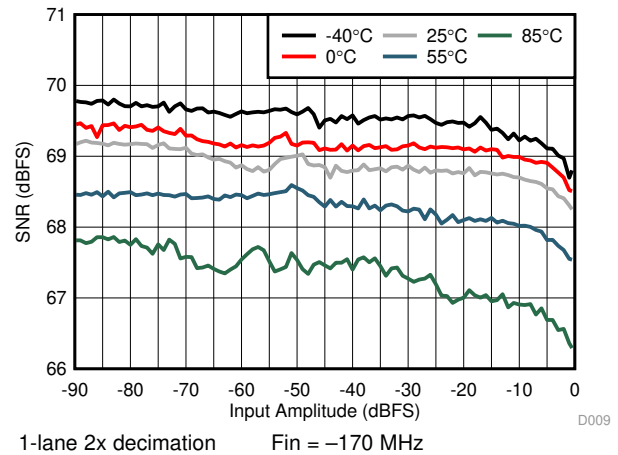
Figure 13. SNR vs. Amplitude
