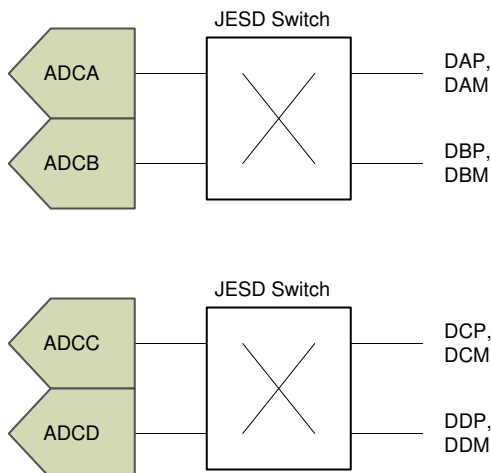
Figure 7-24. Switching the Output Lanes
