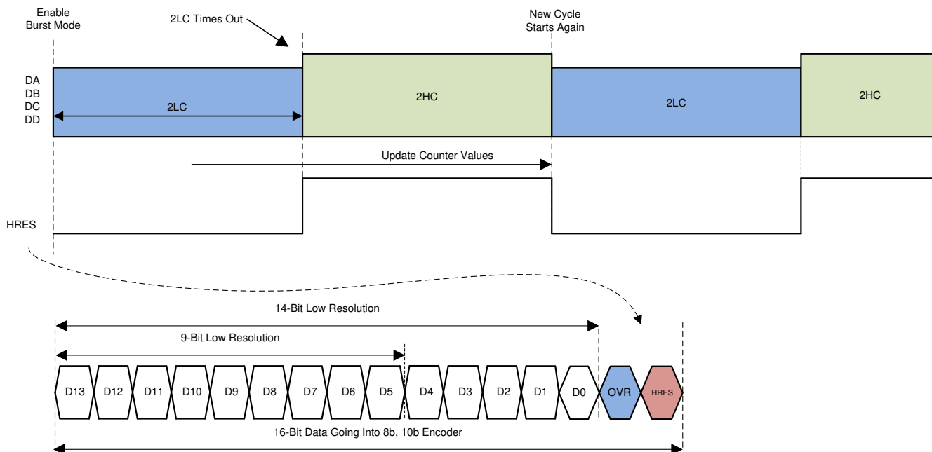
Figure 7-16. Burst Mode
