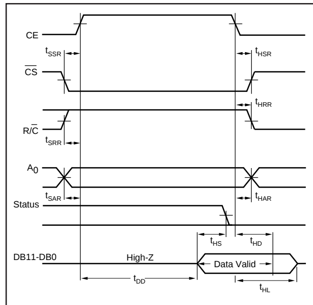
FIGURE 6. Read Cycle Timing.
