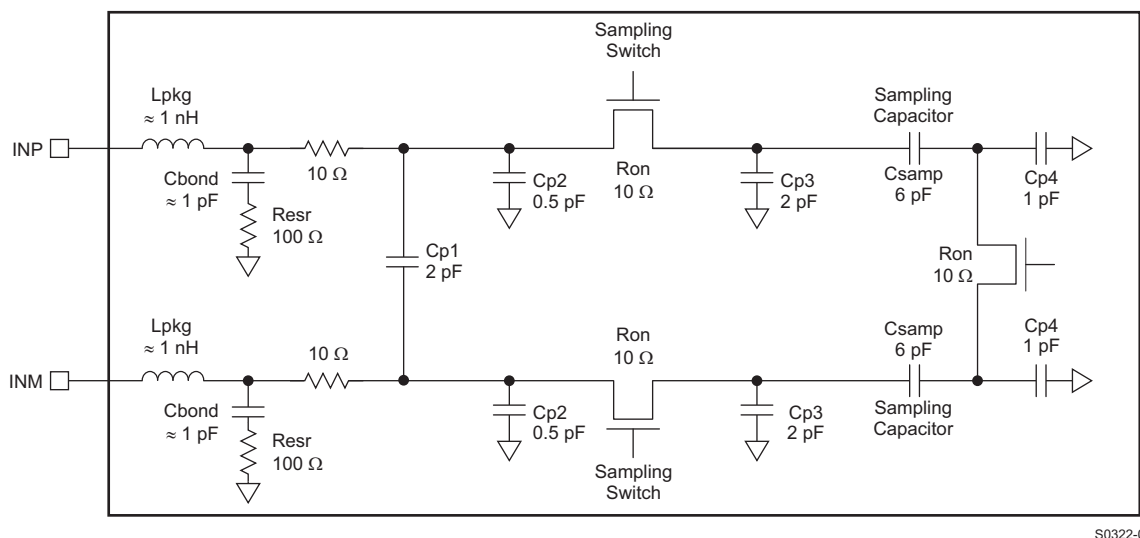
Figure 45. Input Stage
