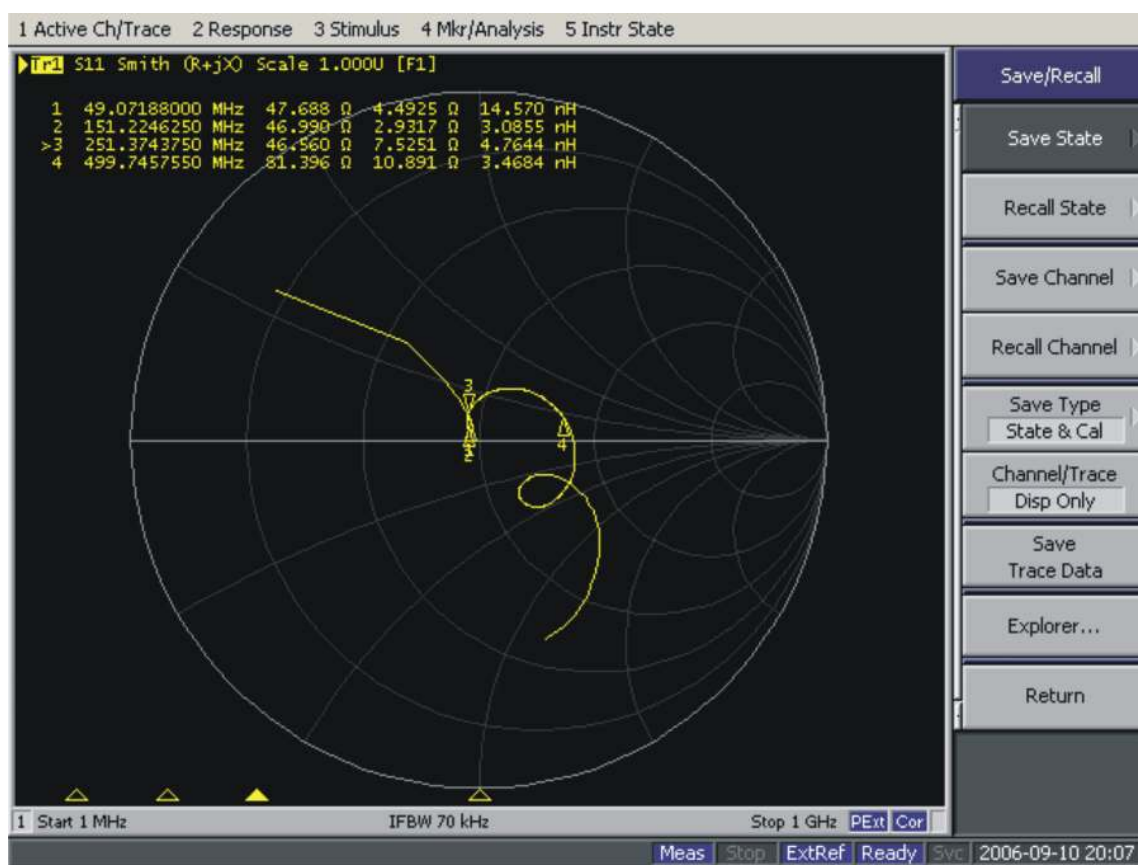
Figure 1. Smith Chart
