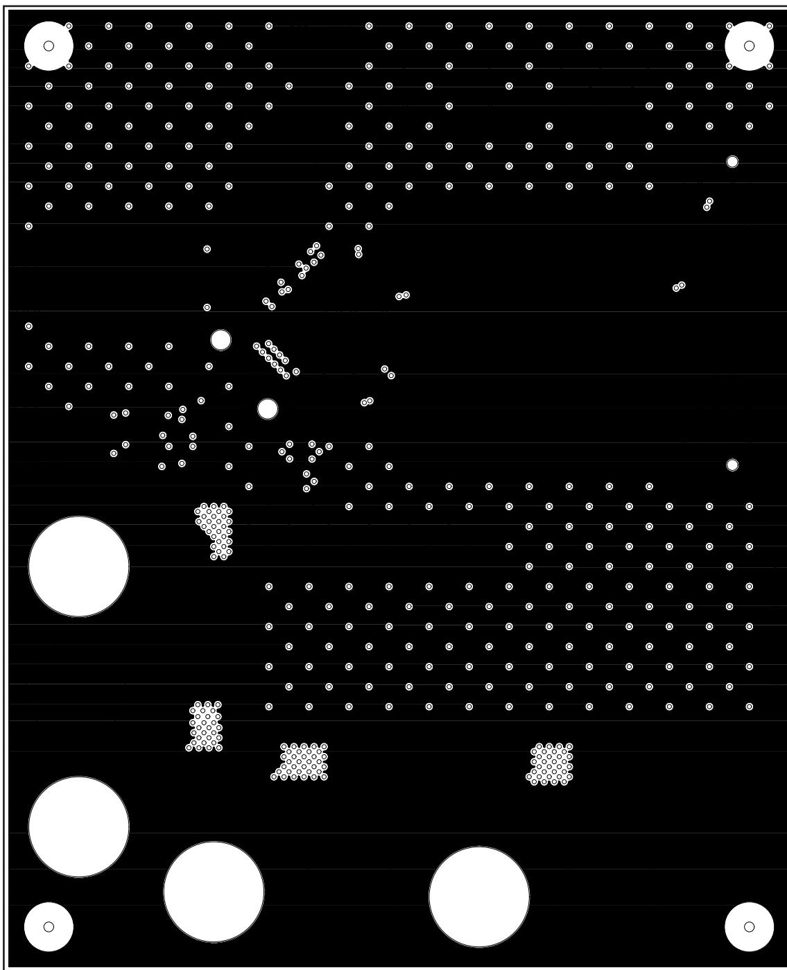
Figure 5. Ground Plane 1
