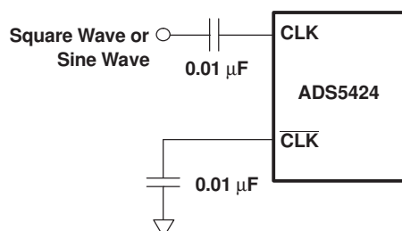
Figure 44. Single-Ended Clock
