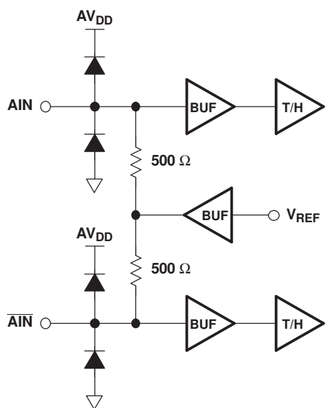
Figure 33. Analog Input
