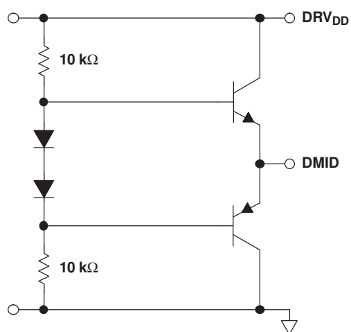
Figure 38. DMID Generation
