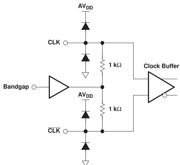
Figure 35. Clock Input
