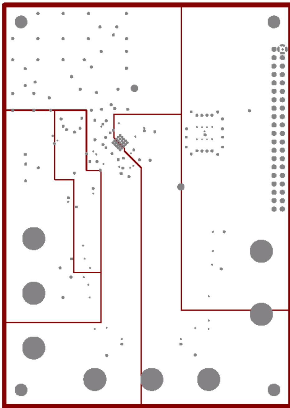
Figure 4-3. Layer 3, Power Plane #1
