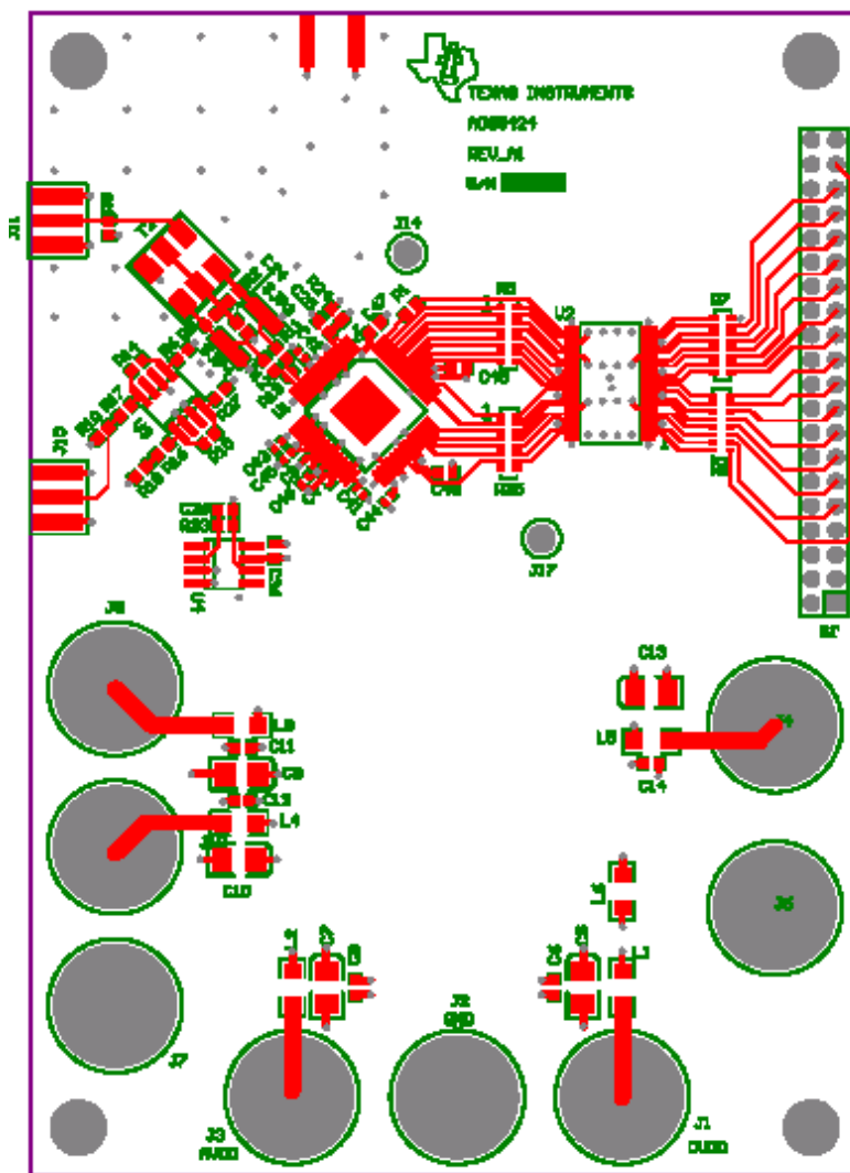
Figure 4-1. Top Layer
