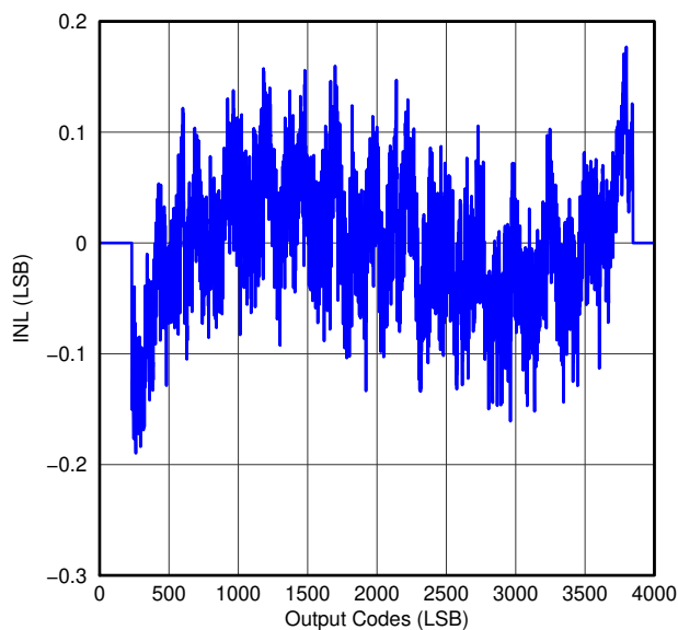
Figure 24. INTEGRAL NONLINEARITY
