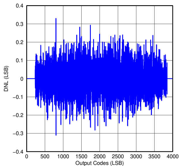
Figure 25. DIFFERENTIAL NONLINEARITY
