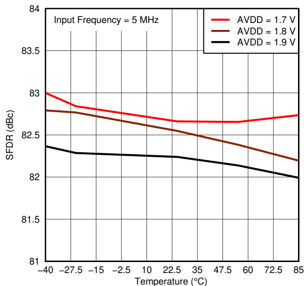
Figure 22. SPURIOUS-FREE DYNAMIC RANGE vs AVDD AND TEMPERATURE
