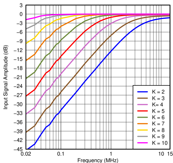
Figure 32. DIGITAL HIGH-PASS FILTER RESPONSE
