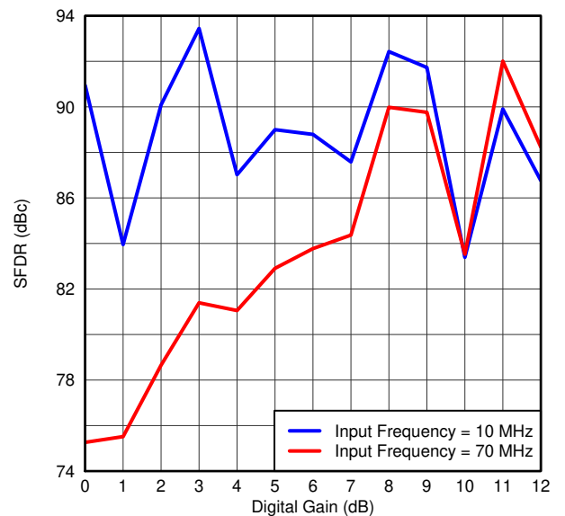
Figure 48. SPURIOUS-FREE DYNAMIC RANGE vs DIGITAL GAIN
