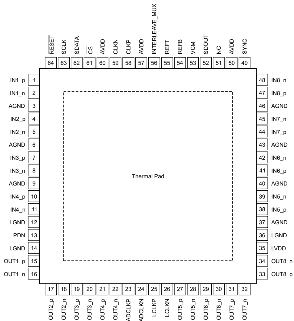
RGC PACKAGE QFN-64 (Top View)
