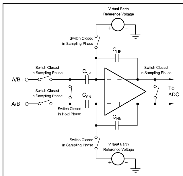
Figure 6. SHA/SHPGA Architecture.
