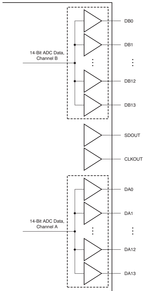
Figure 42. CMOS Outputs
