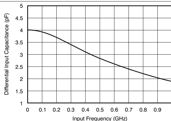
Figure 73. ADC Analog Input Capacitance ( C_{IN} ) Across Frequency
