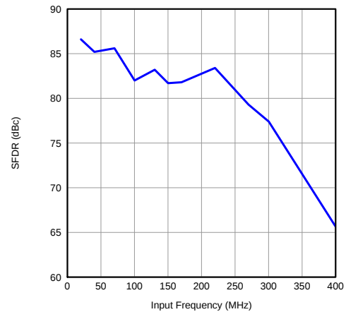
Figure 68. SFDR vs Input Frequency
