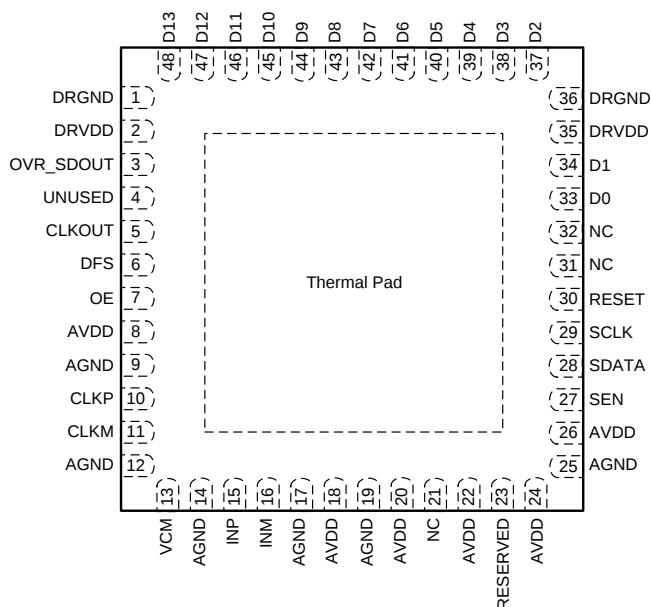
ADS414x RGZ Package 48-PIN VQFN With Exposed Thermal Pad CMOS Mode -Top View
