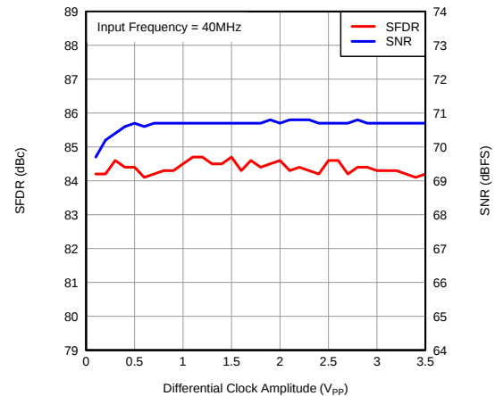
Figure 40. Performance Across Input Clock Amplitude
