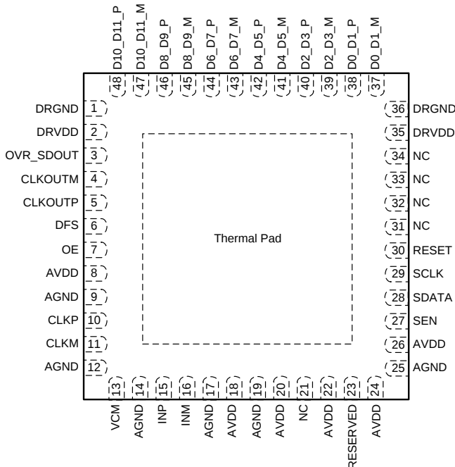
ADS412x RGZ Package 48-Pin VQFN With Exposed Thermal Pad LVDS Mode - Top View
