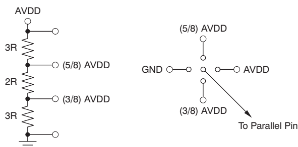
Figure 103. Simplified Diagram to Configure DFS Pin
