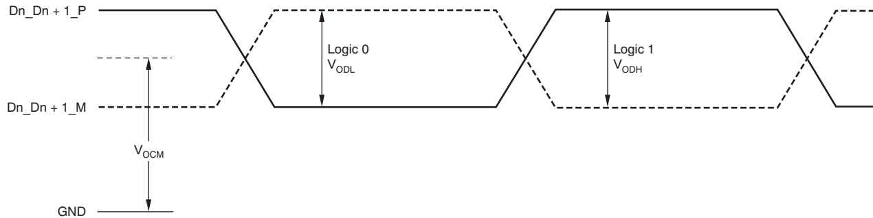
Figure 7. LVDS Output Voltage Levels
