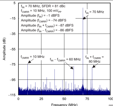
Figure 27. CMRR Spectrum
