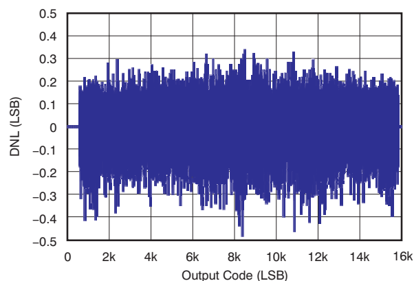
DIFFERENTIAL NONLINEARITY
