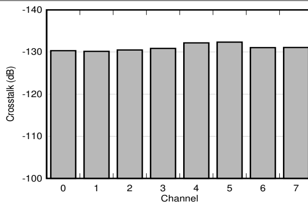
Figure 6-23. Crosstalk vs Channel
