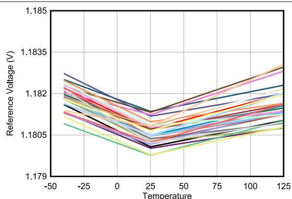
Figure 6-29. Internal Reference Voltage Temperature Drift
