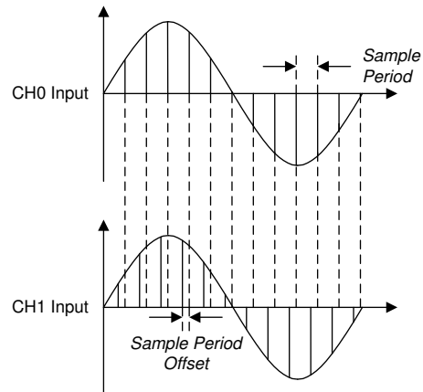
Figure 8-10. Channel 1 With a Positive Sample Phase Shift With Respect to Channel 0
