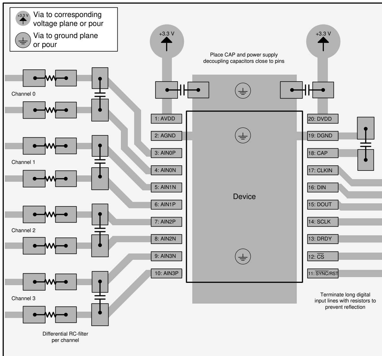
Figure 9-6. Layout Example
