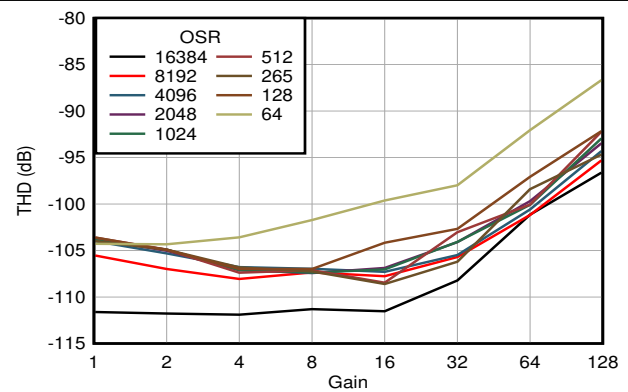
Figure 6-25. THD vs Gain
