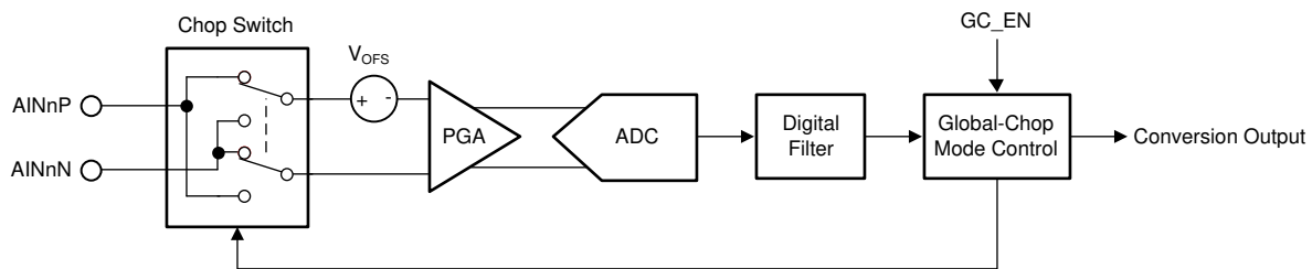
Figure 8-15. Global-Chop Mode Implementation
