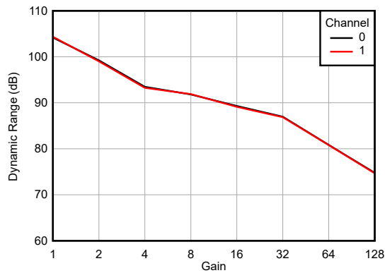
Figure 6-22. Dynamic Range vs Gain
