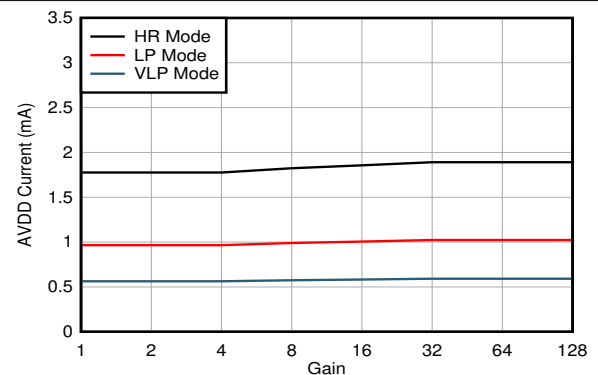
Figure 6-27. AVDD Current vs Gain
