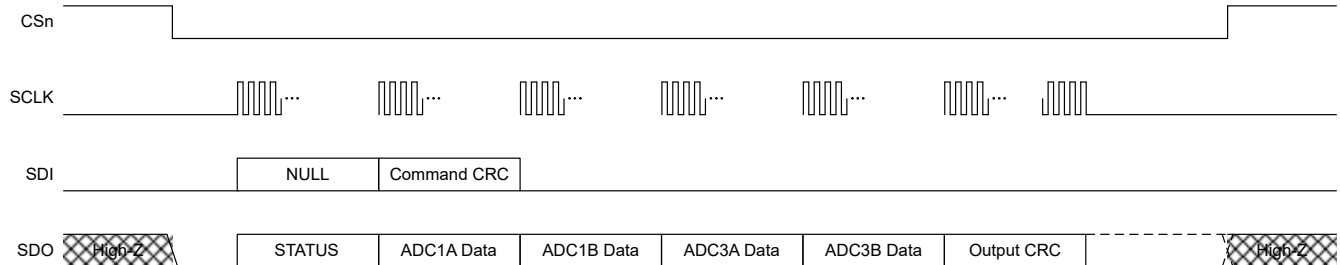
Figure 7-28. Typical Communication Frame
