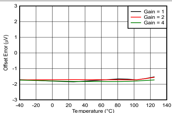
Figure 5-15. ADC3y Offset Error vs Temperature
