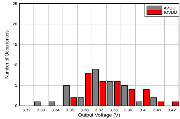
Figure 5-39. AVDD and IOVDD LDO Output Voltage Histogram
