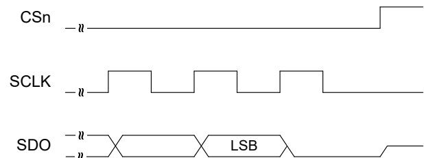
Figure 7-25. SDO Behavior With Additional SCLK Pulses
