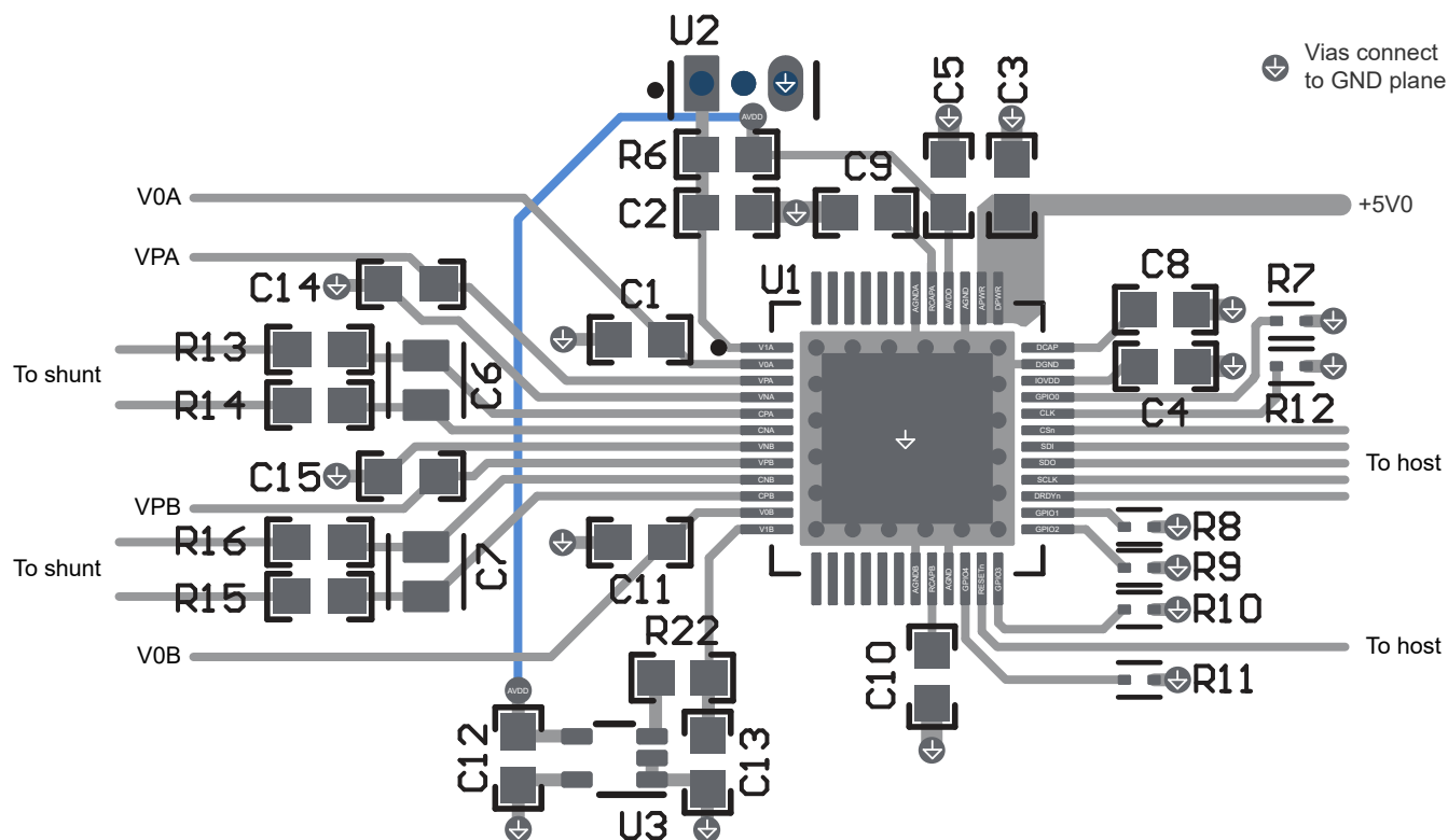
Figure 9-8. Layout Example
