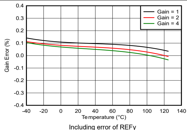
Figure 5-11. ADC2A Gain Error vs Temperature
