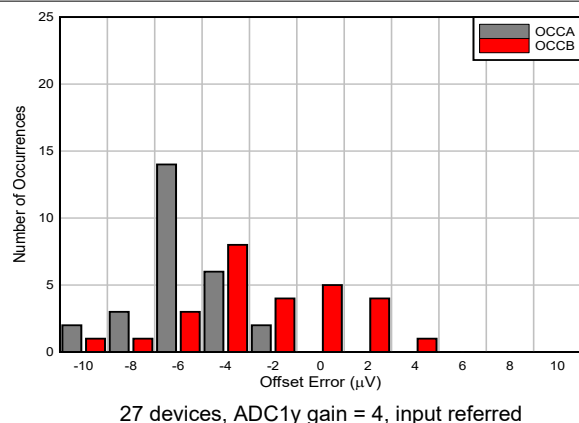
Figure 5-16. OCCy Offset Error Histogram
