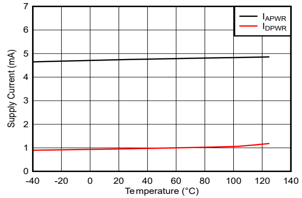
Figure 5-35. Supply Current vs Temperature Active mode, all ADCs enabled and converting
