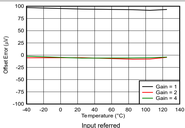
Figure 5-9. ADC2A Offset Error vs Temperature
