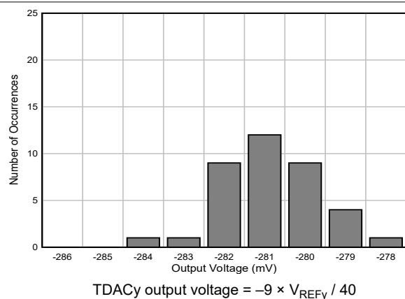
Figure 5-24. Test DACy Output Voltage Histogram
