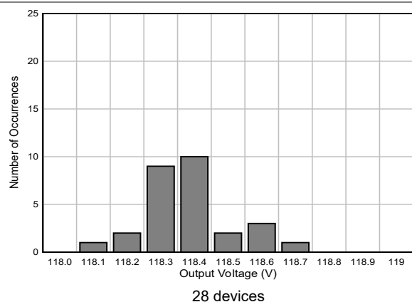
Figure 5-20. Temperature Sensor Output Voltage Histogram
