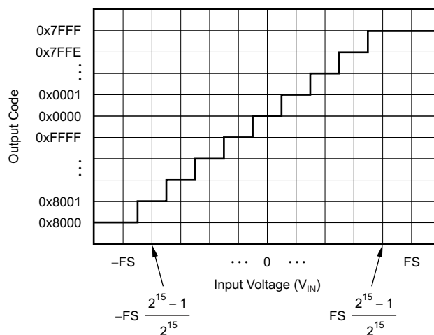
Figure 7-12. Code Transition Diagram (16-Bit Conversion Data)
