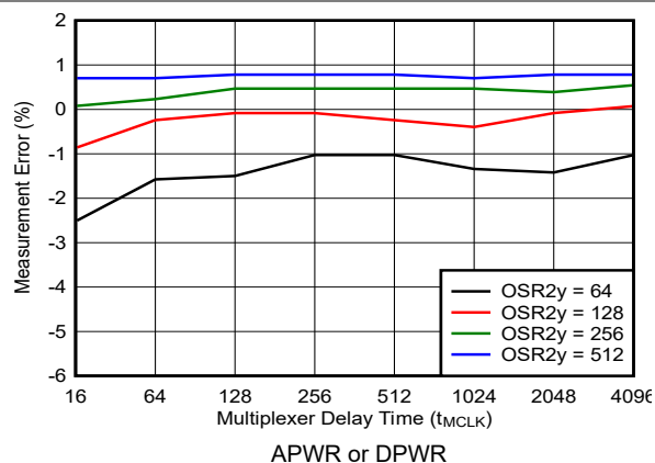
Figure 5-26. ADC2A Supply Voltage Readback Measurement Accuracy
