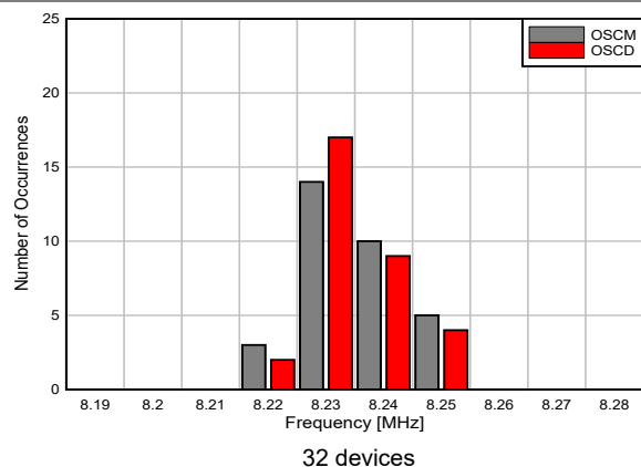
Figure 5-14. OSCM and OSCD Frequency Histogram
