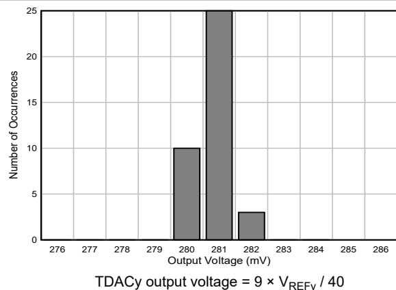
Figure 5-22. Test DACy Output Voltage Histogram
