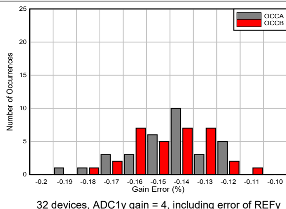
Figure 5-18. OCCy Gain Error Histogram
