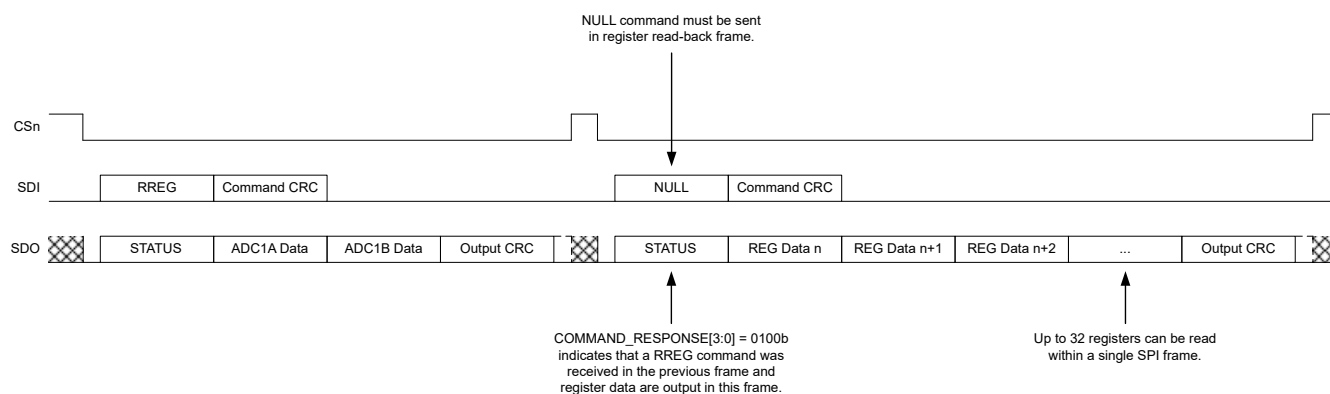
Figure 7-37. RREG Command Frame
