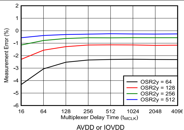
Figure 5-27. ADC2A Supply Voltage Readback Measurement Accuracy
