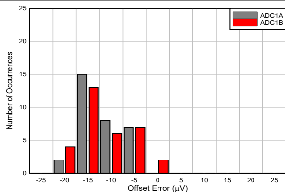
Figure 5-2. ADC1y Offset Error Histogram
