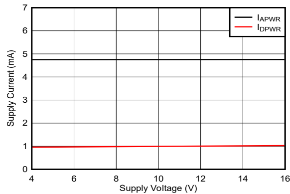
Figure 5-36. Supply Current vs Supply Voltage Active mode, all ADCs enabled and converting
