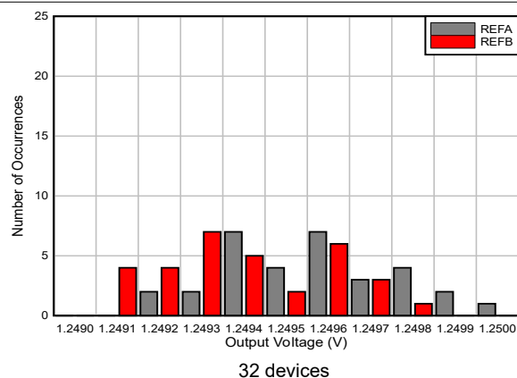
Figure 5-12. REFy Output Voltage Histogram
