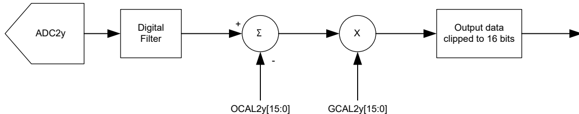
Figure 7-8. Calibration Logic Block Diagram
