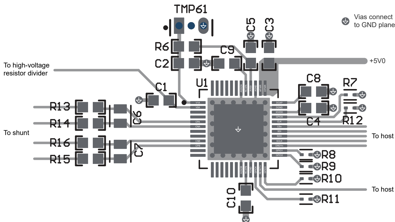
Figure 9-8. Layout Example
