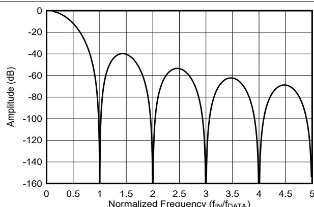
Figure 7-3. Sinc3 Filter Frequency Response
