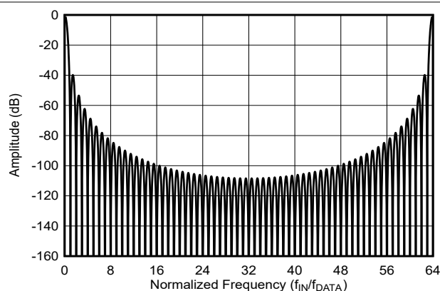
Figure 7-4. Sinc3 Filter Frequency Response to f_{MOD} (OSR = 64)
