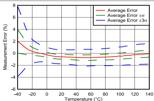
Figure 5-21. Temperature Sensor Measurement Error vs Ambient Temperature
